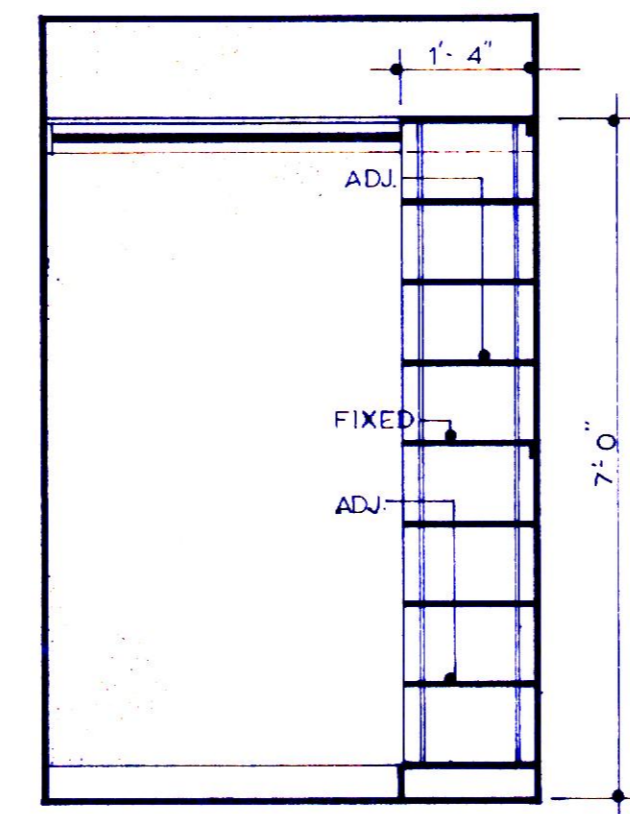
ELEVATION AT 10
