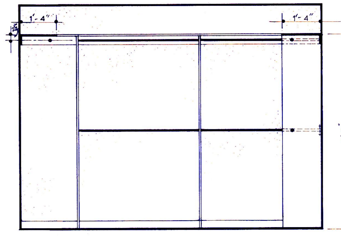
ELEVATION AT 5
