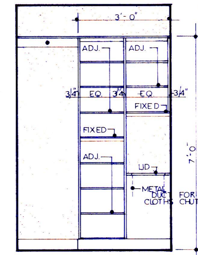
ELEVATION AT 11
