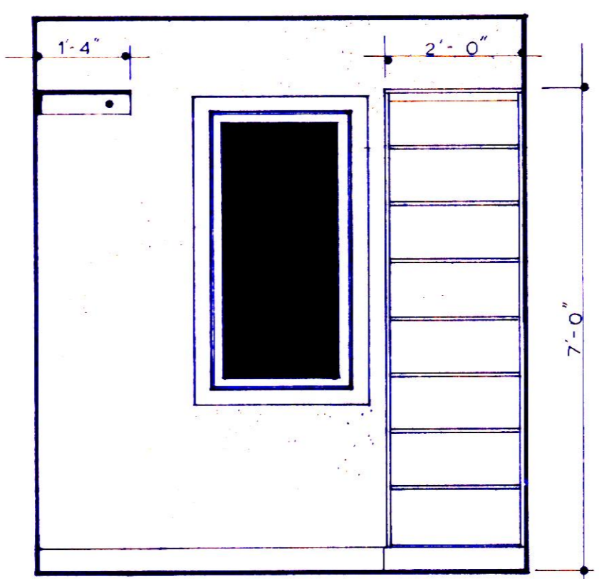
ELEVATION AT 8
