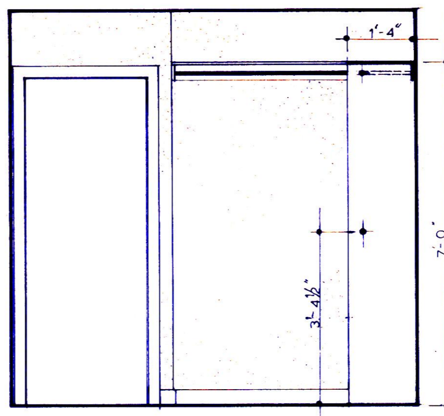
ELEVATION AT 4
