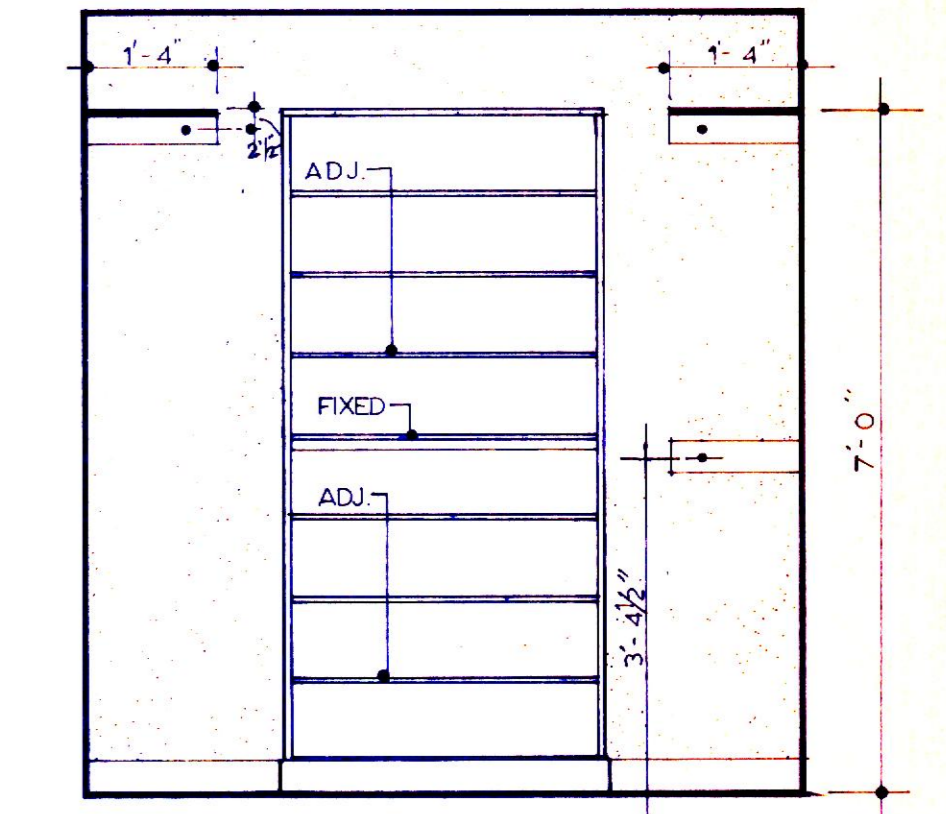
ELEVATION AT 14
