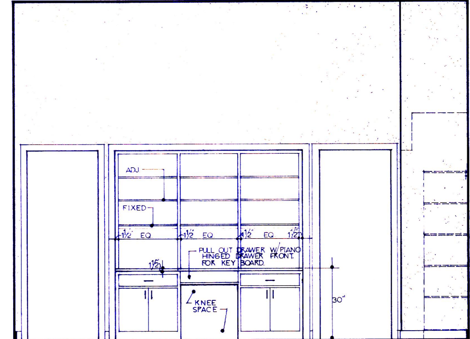
ELEVATION AT 12
