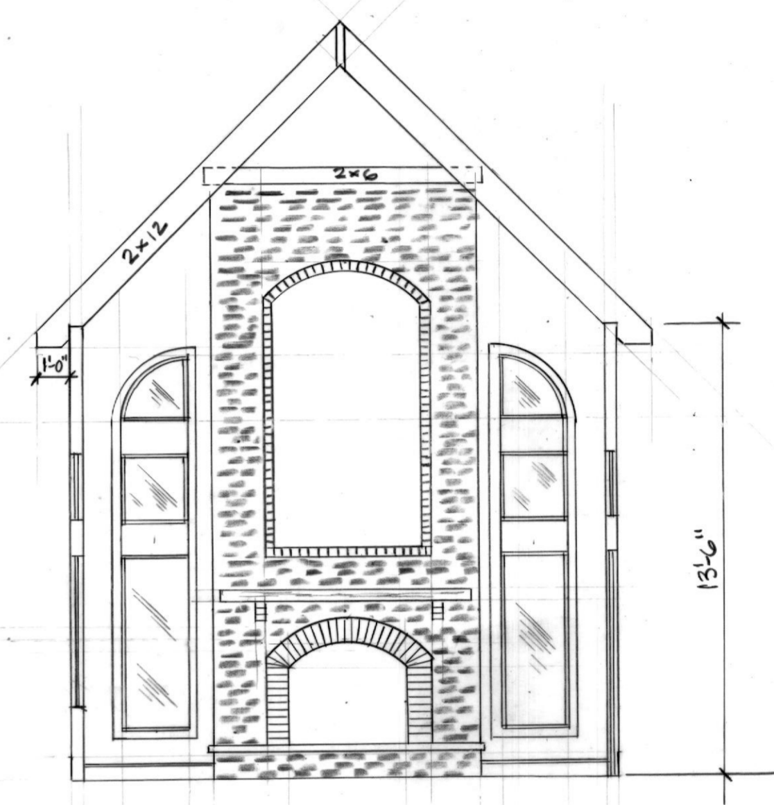
FAMILY ROOM SECTION
