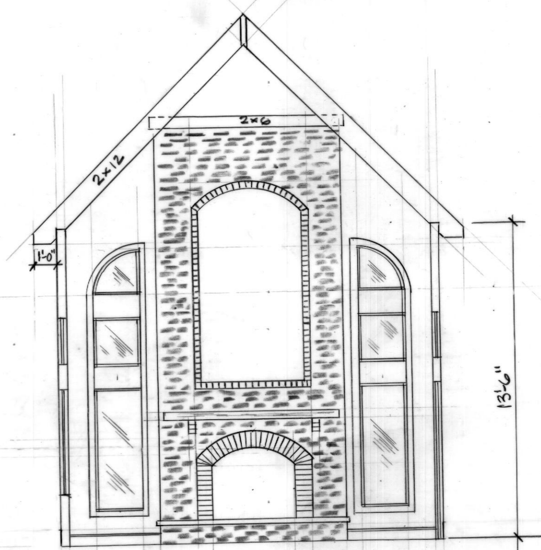
FAMILY ROOM SECTION
