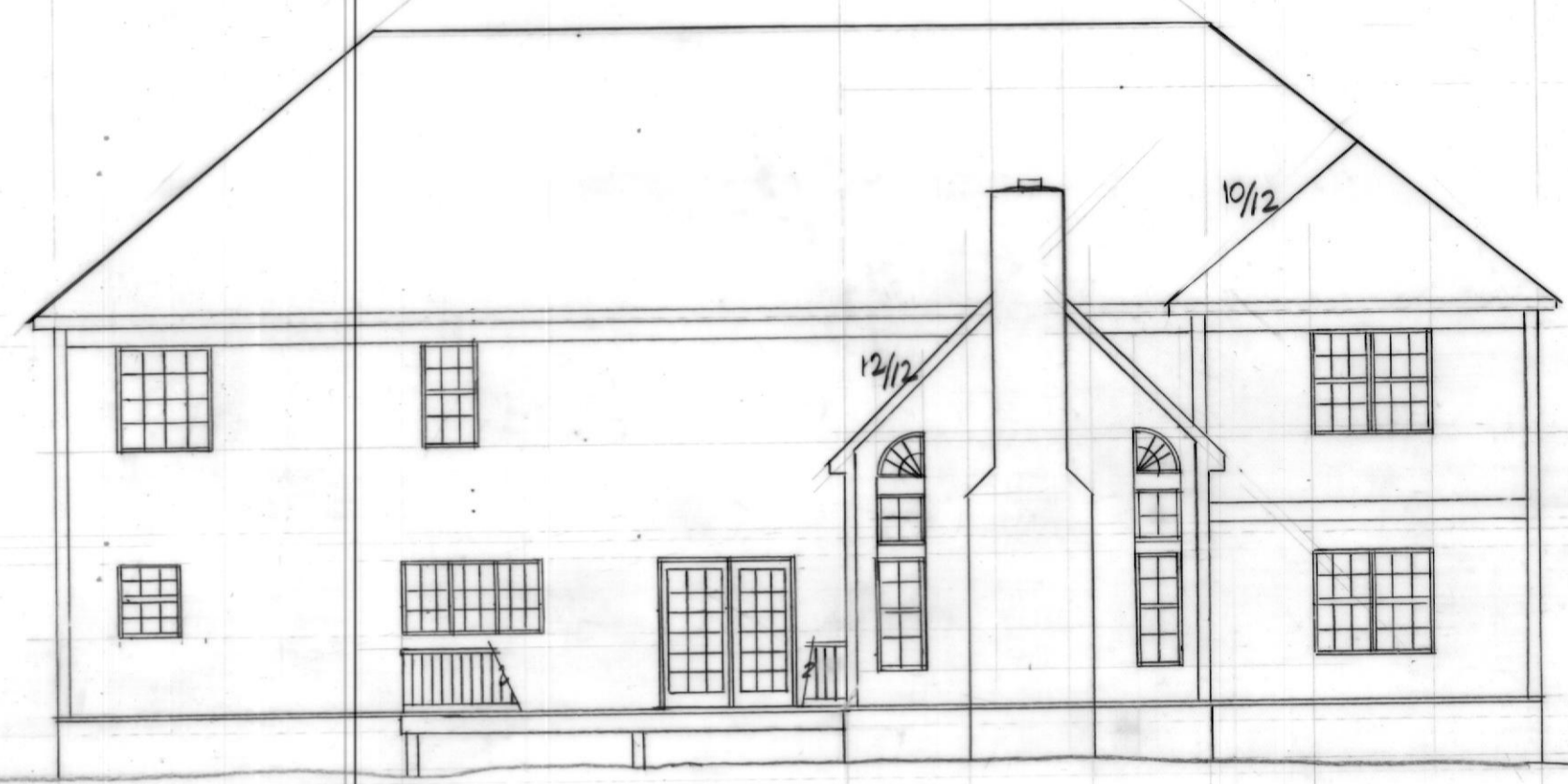
REAR ELEVATION
