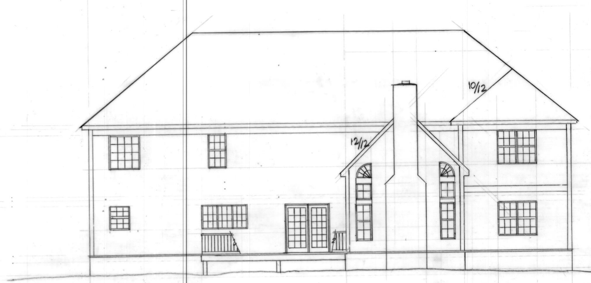
REAR ELEVATION
