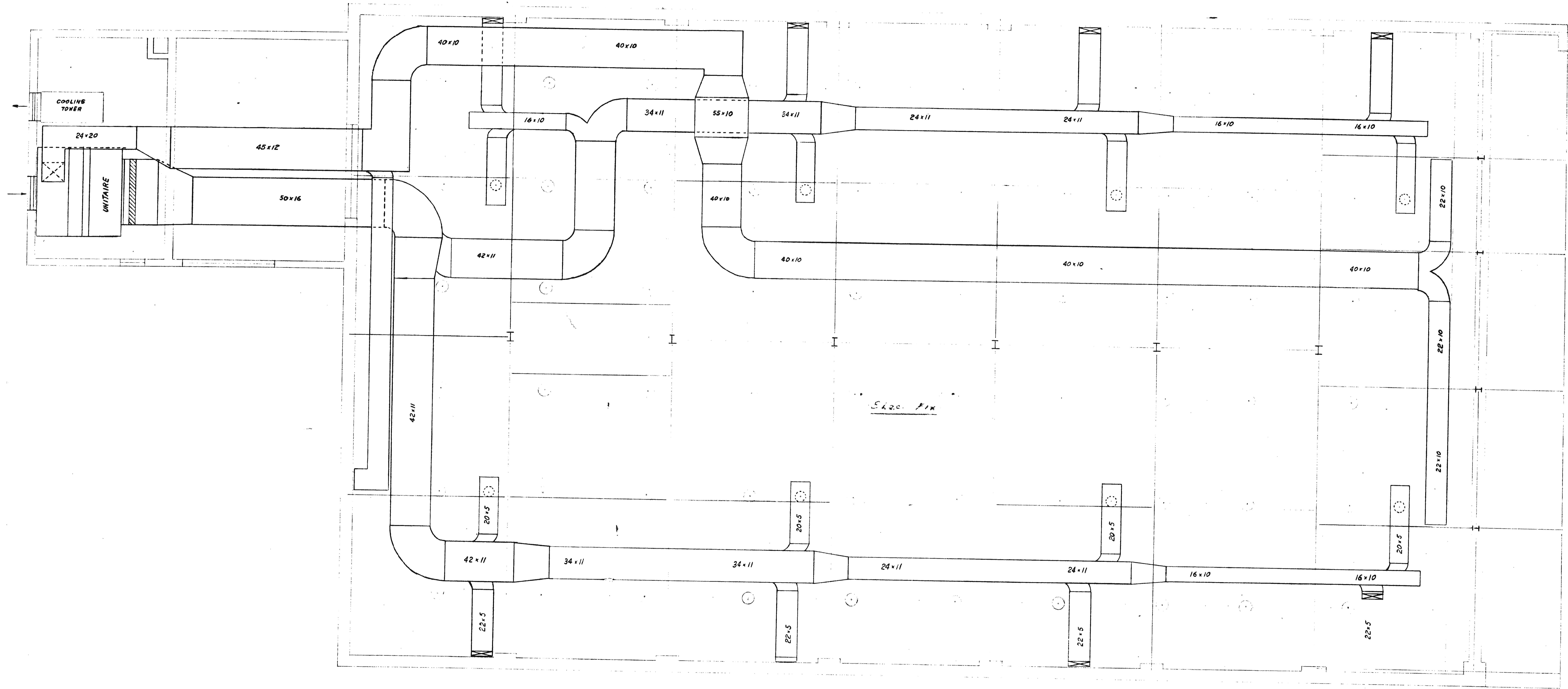
HEATING & AIR CONDITIONING LAYOUT for CARTERS FURNITURE STORE, TOWSON MD
