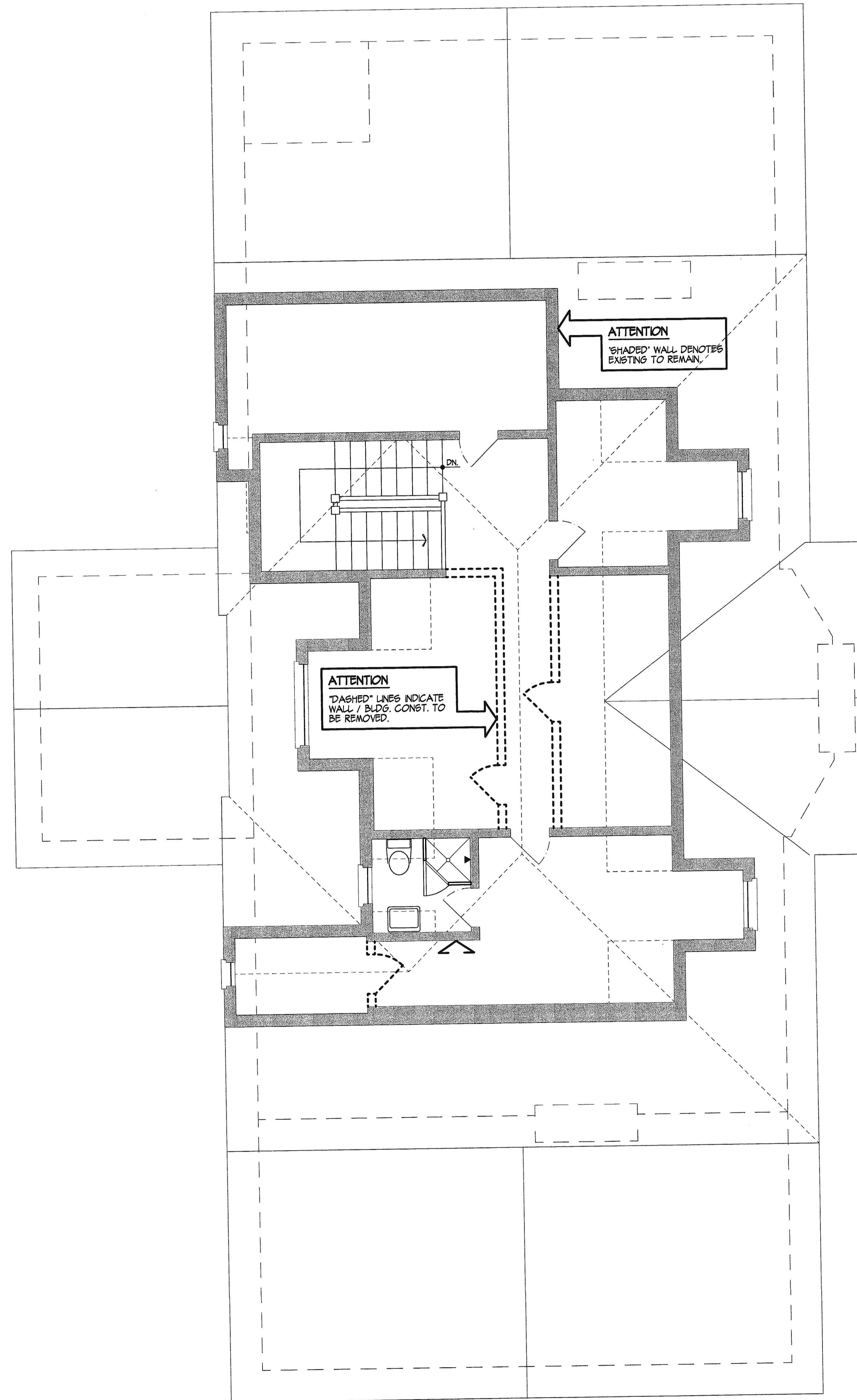
THIRD FLOOR DEMOLITION PLAN SCALE: 1/4"=1'-0"
