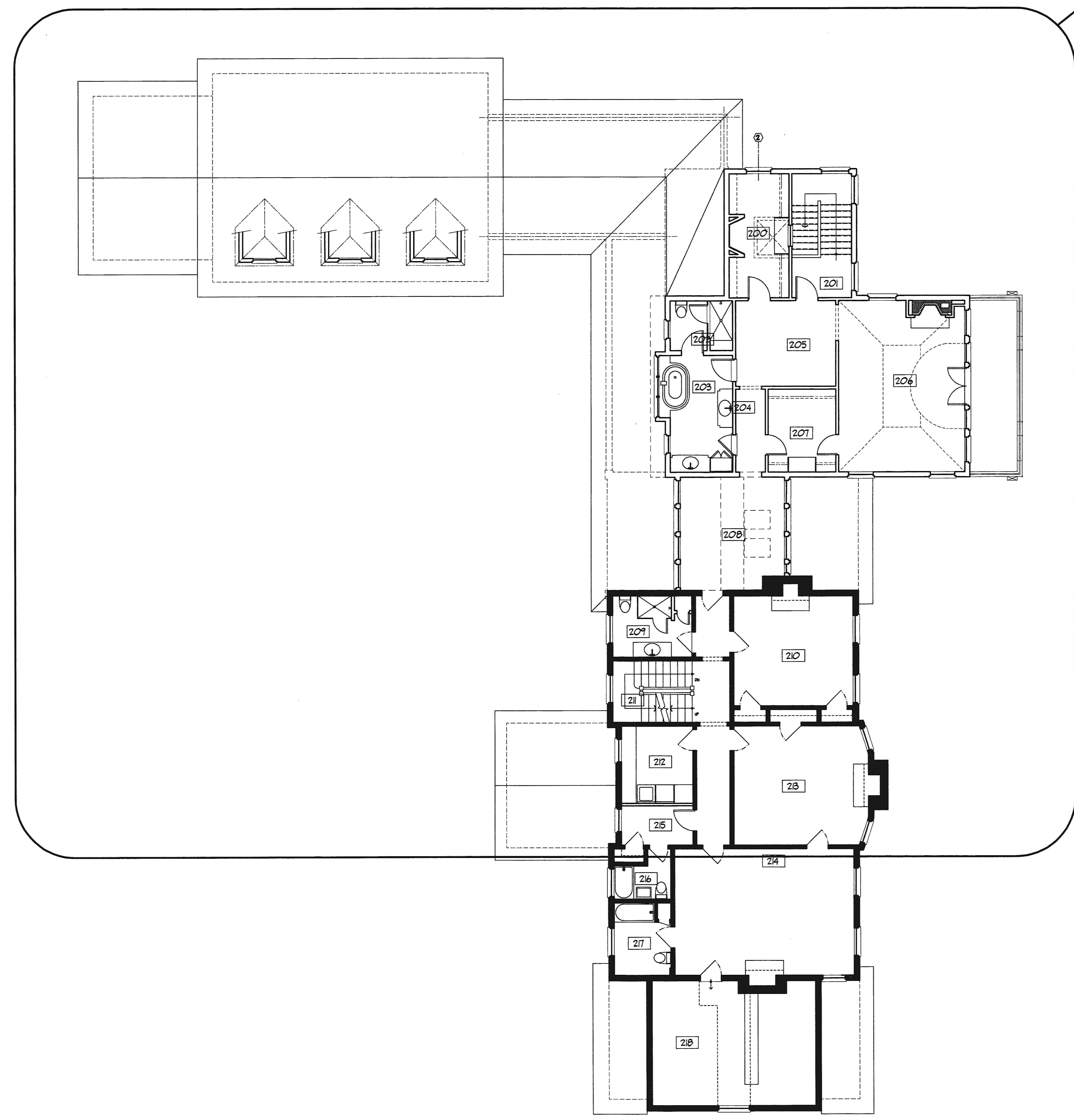
SECOND FLOOR COORDINATION PLAN SCALE: 1/8"=1'-0"
