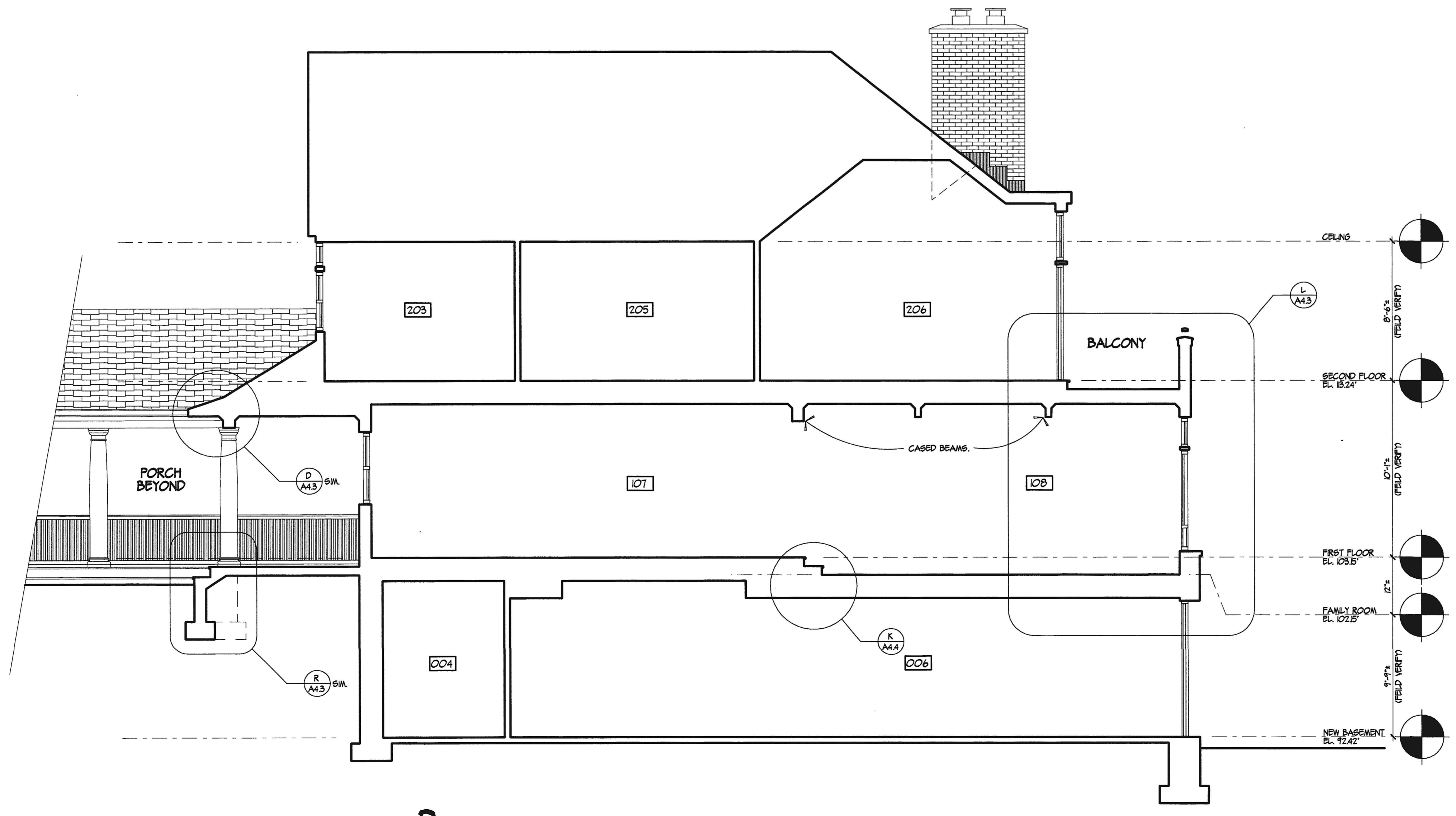
BUILDING SECTION B SCALE: 1/4"=1'-0"
