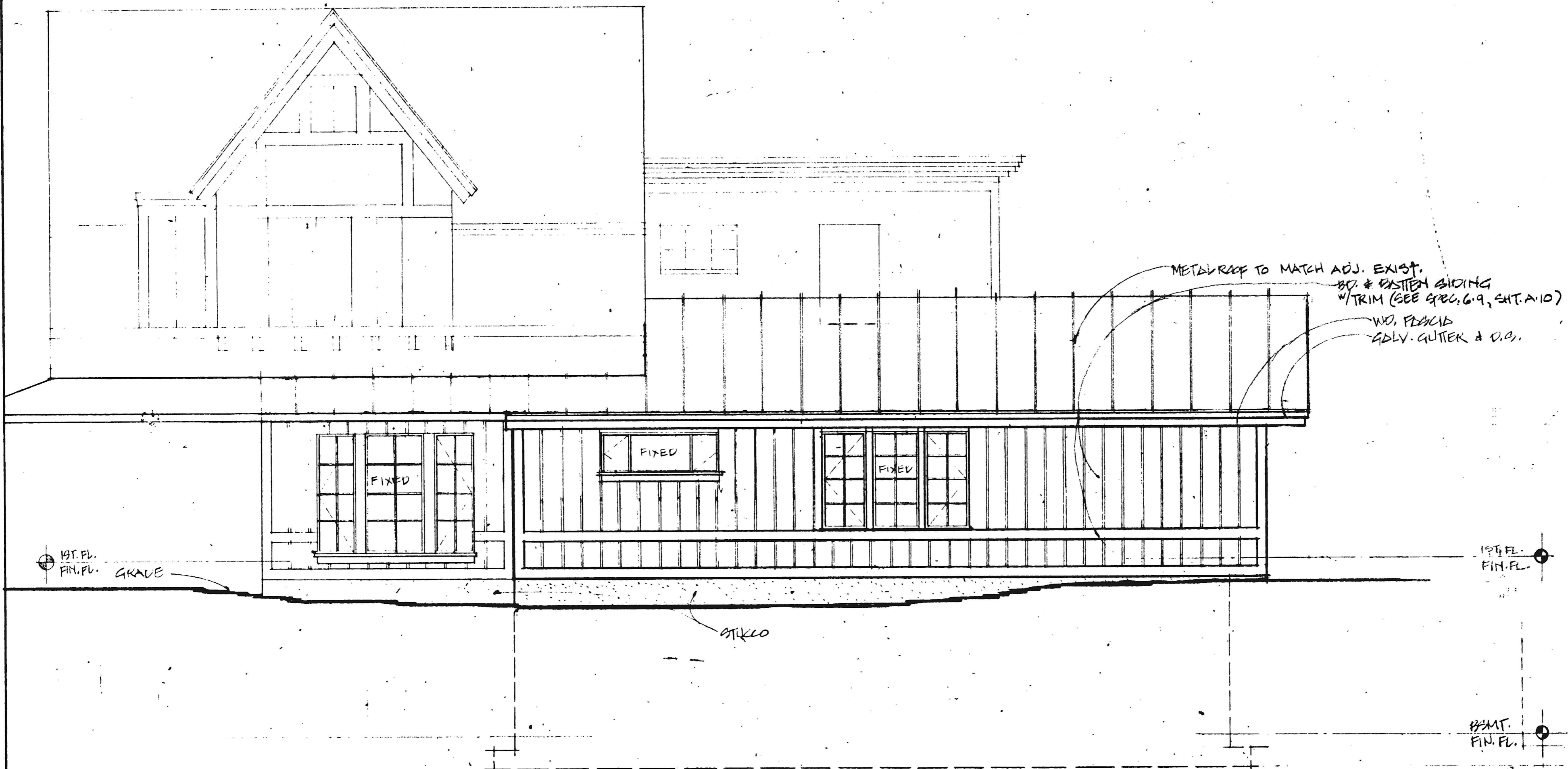
WEST ELEVATION 1/4" = 1'-0"
