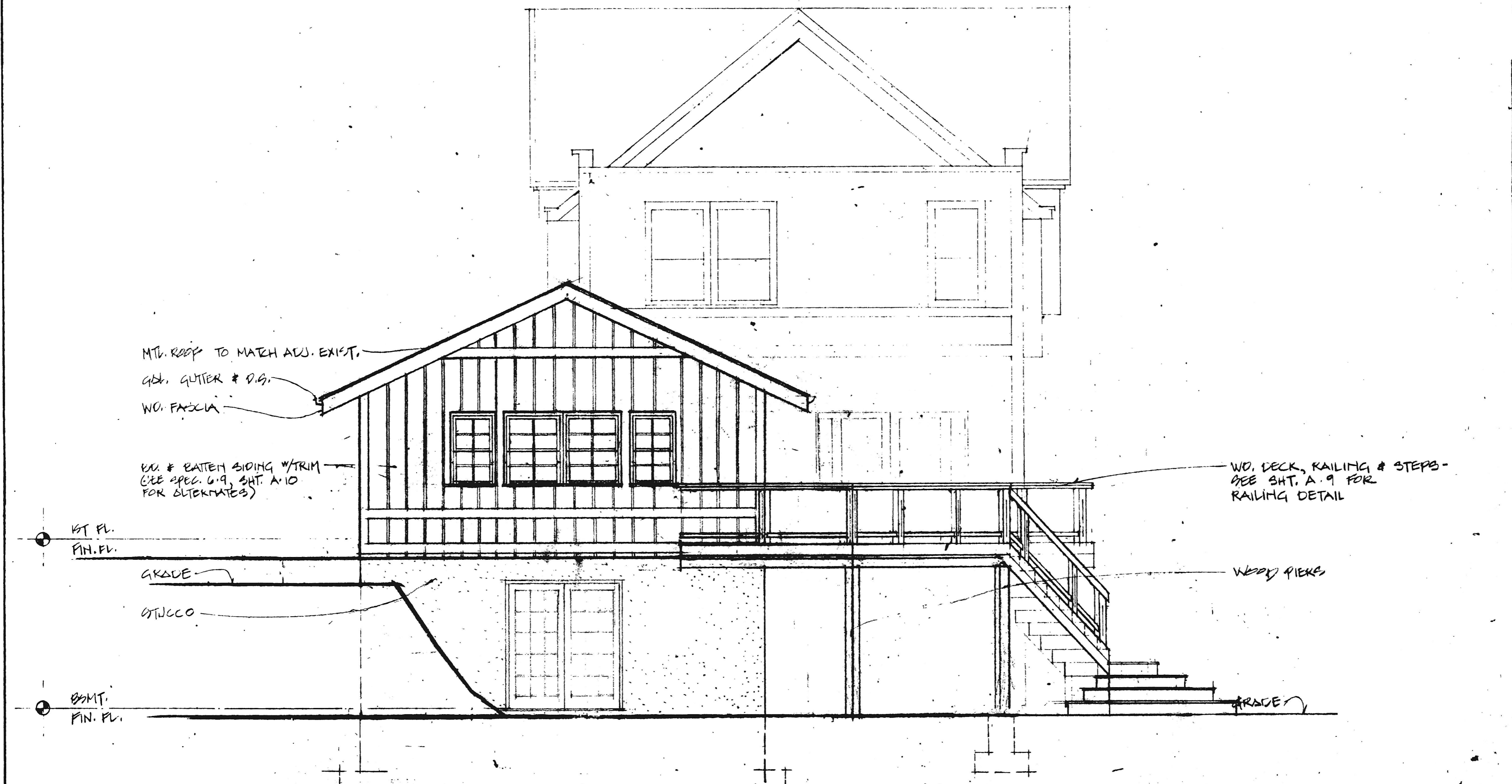
SOUTH - ELEVATION 1/4" = 1'-0"
