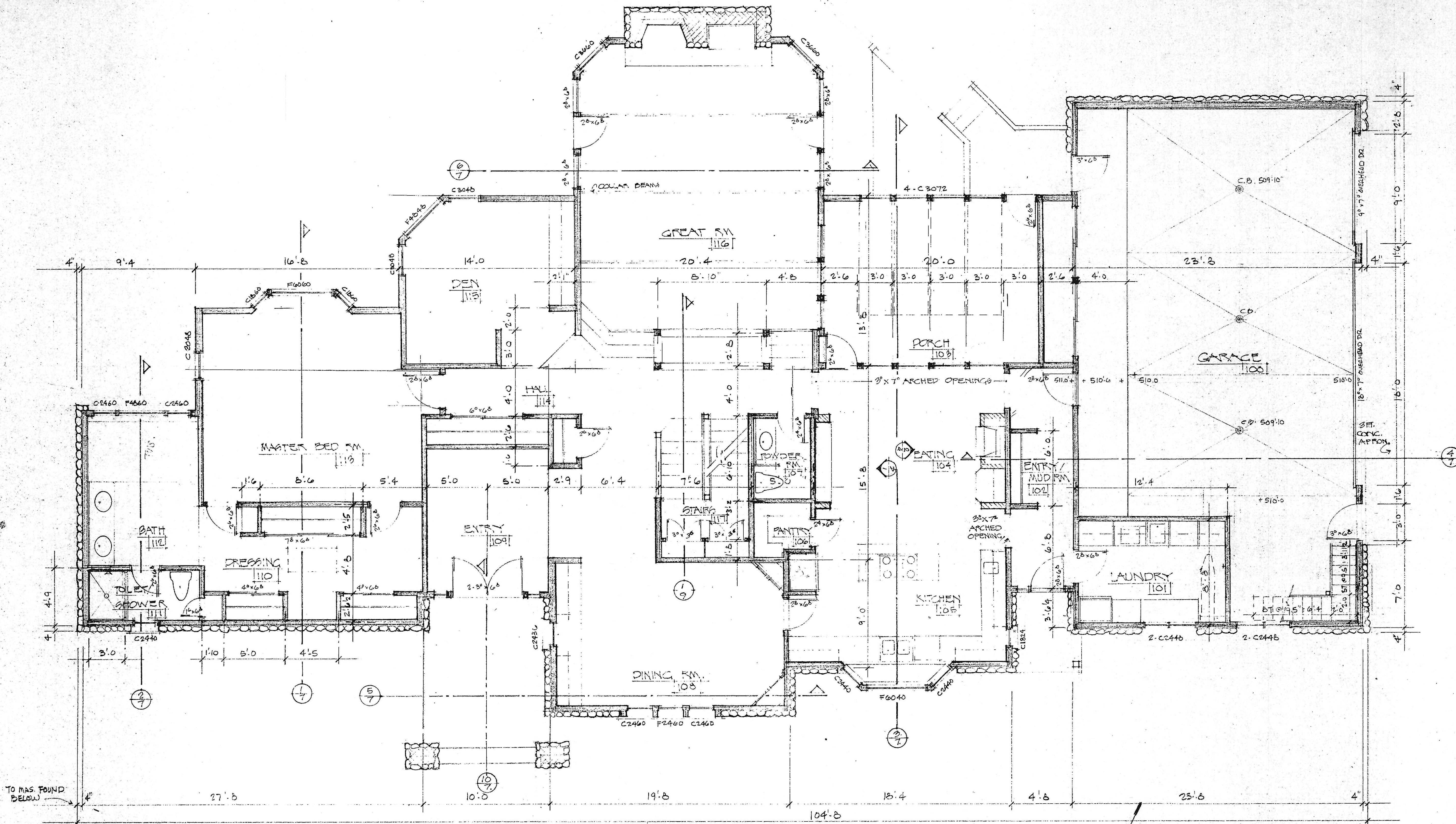
MAIN LEVEL FLOOR PLAN SCALE: 1/4" = 1'-0"
