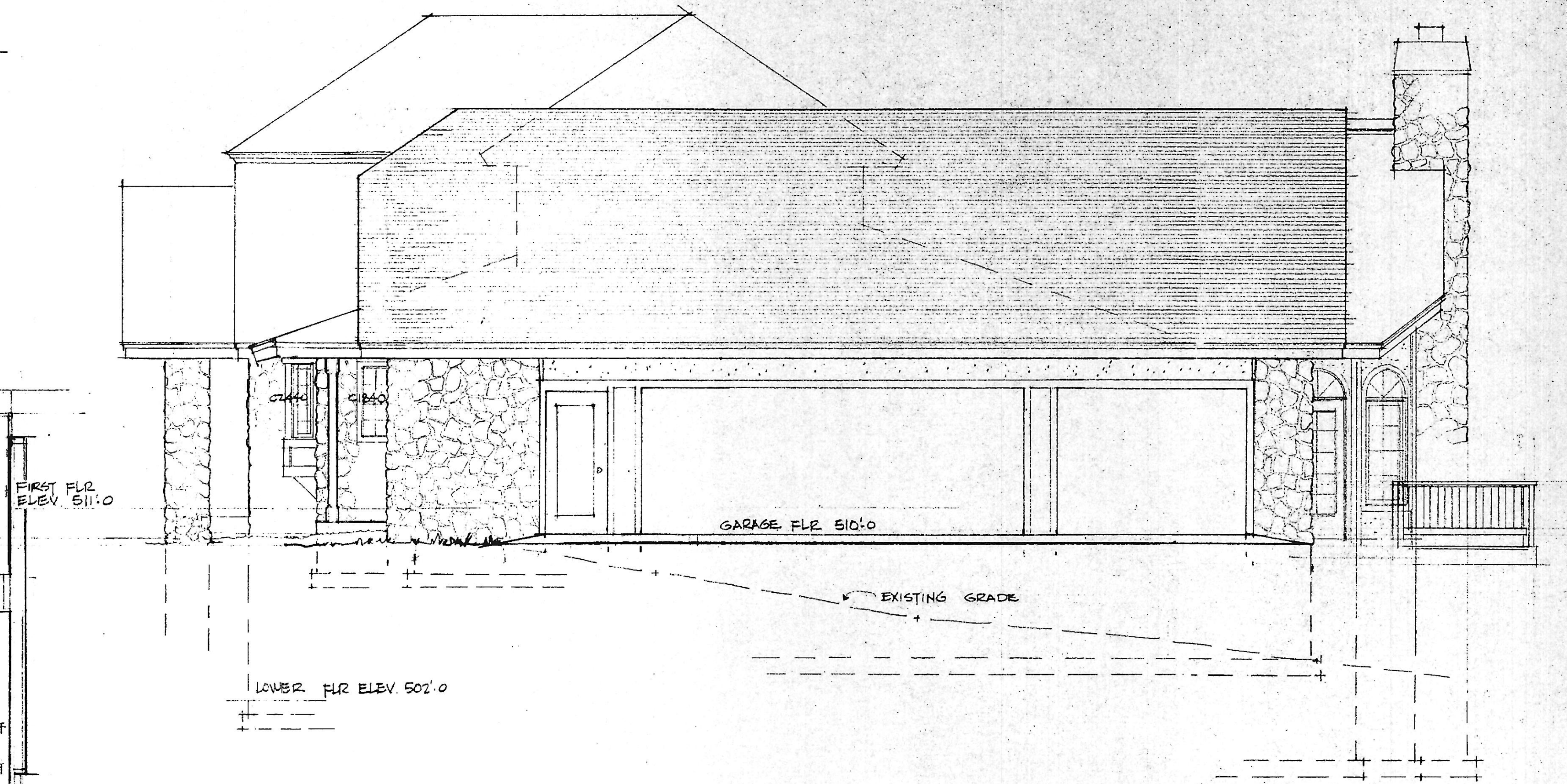
EAST ELEV.
