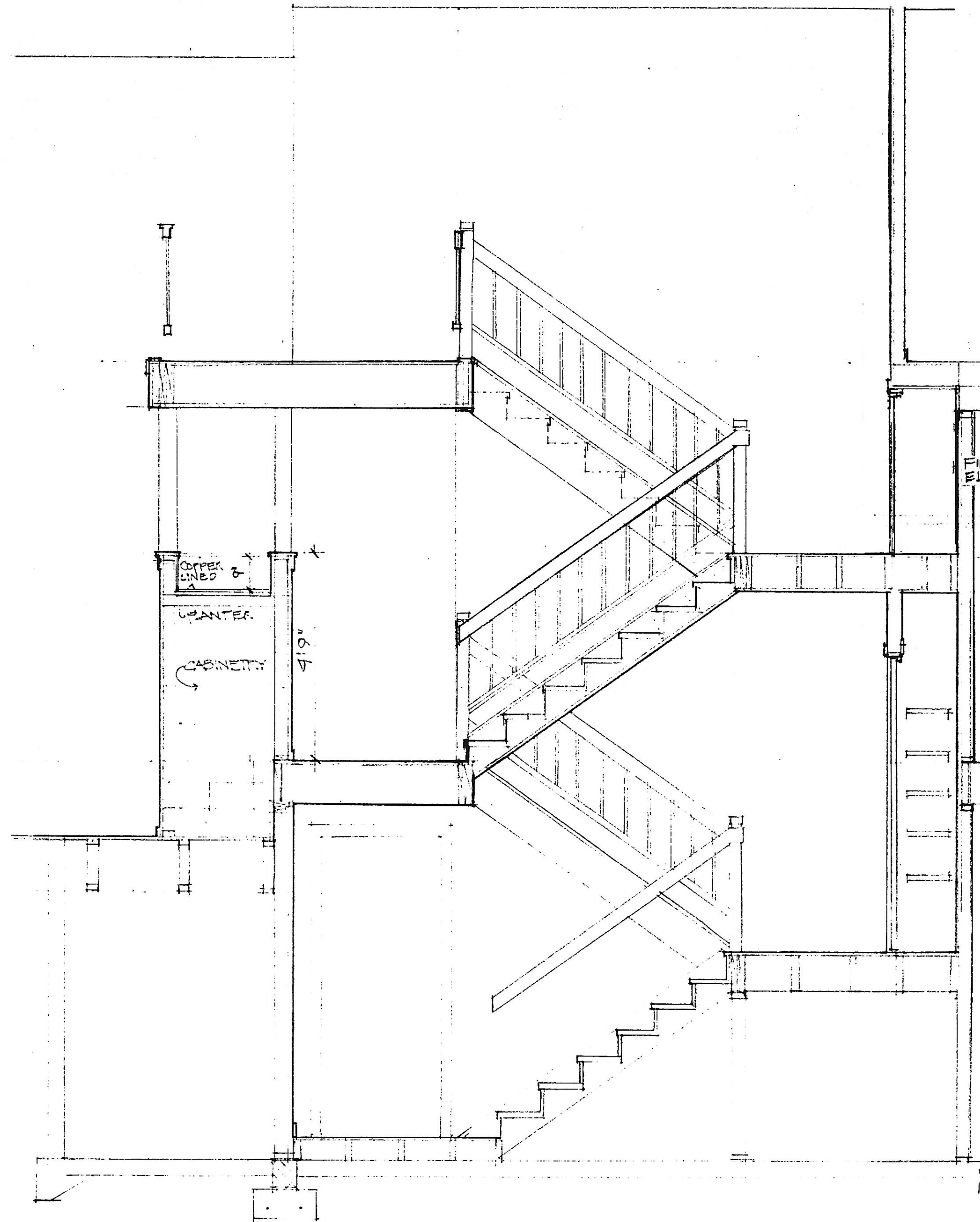
1. STAR SECTION a. SCALE 1/2" = 1'-0"
