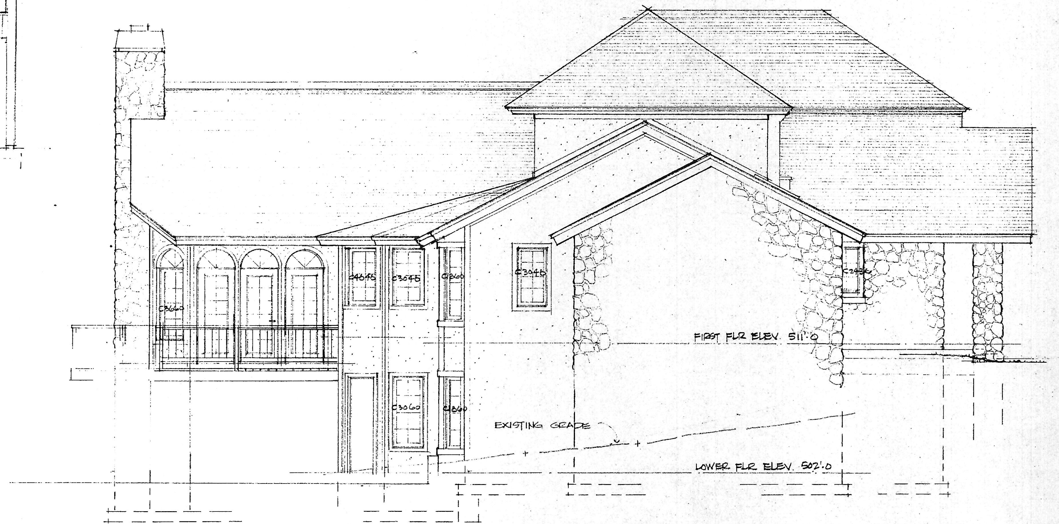
WEST ELEV. SCALE 1/4" = 1'-0"
