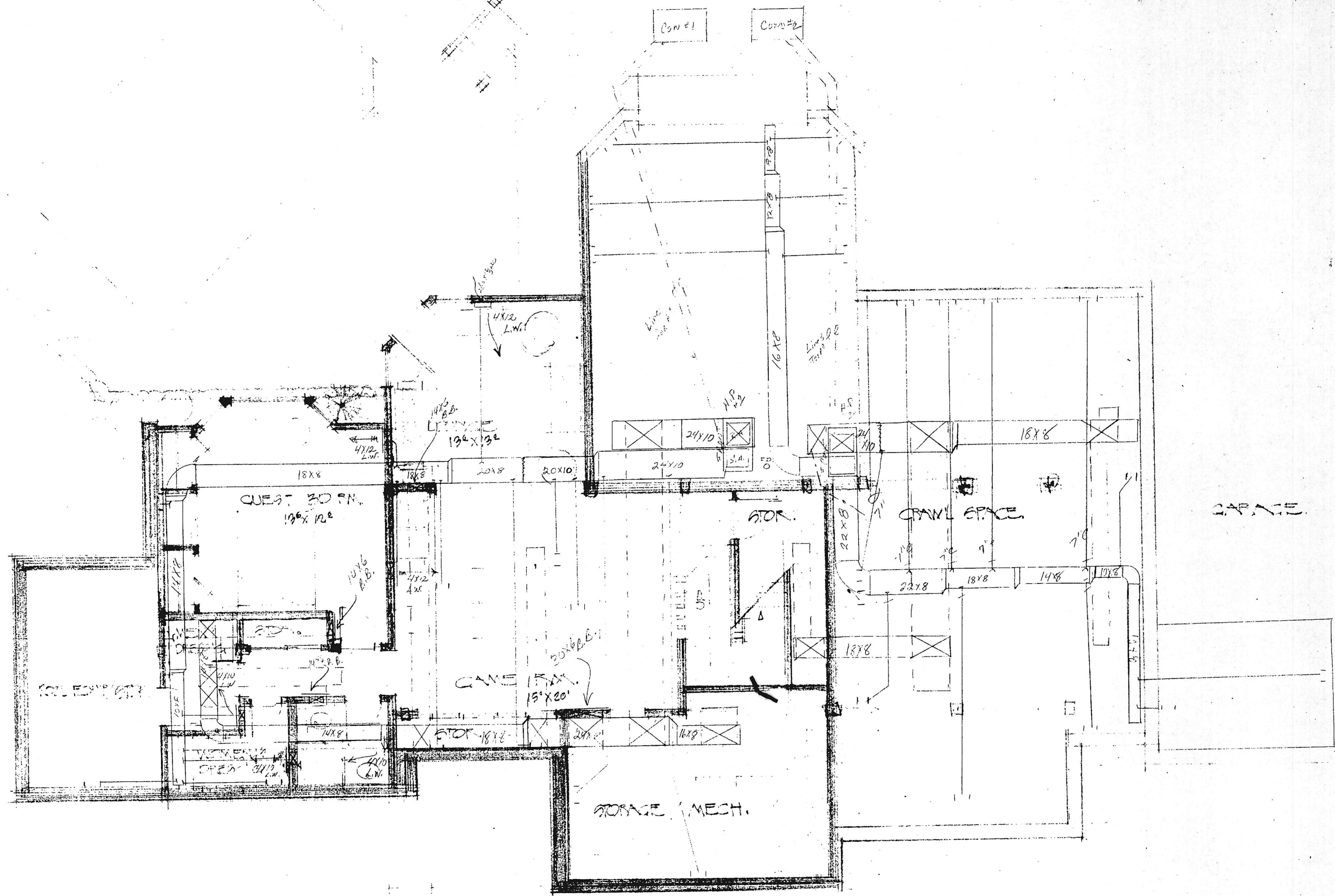
LOWER LEVEL PLAN SCALE: 1/4" = 1'-0"
