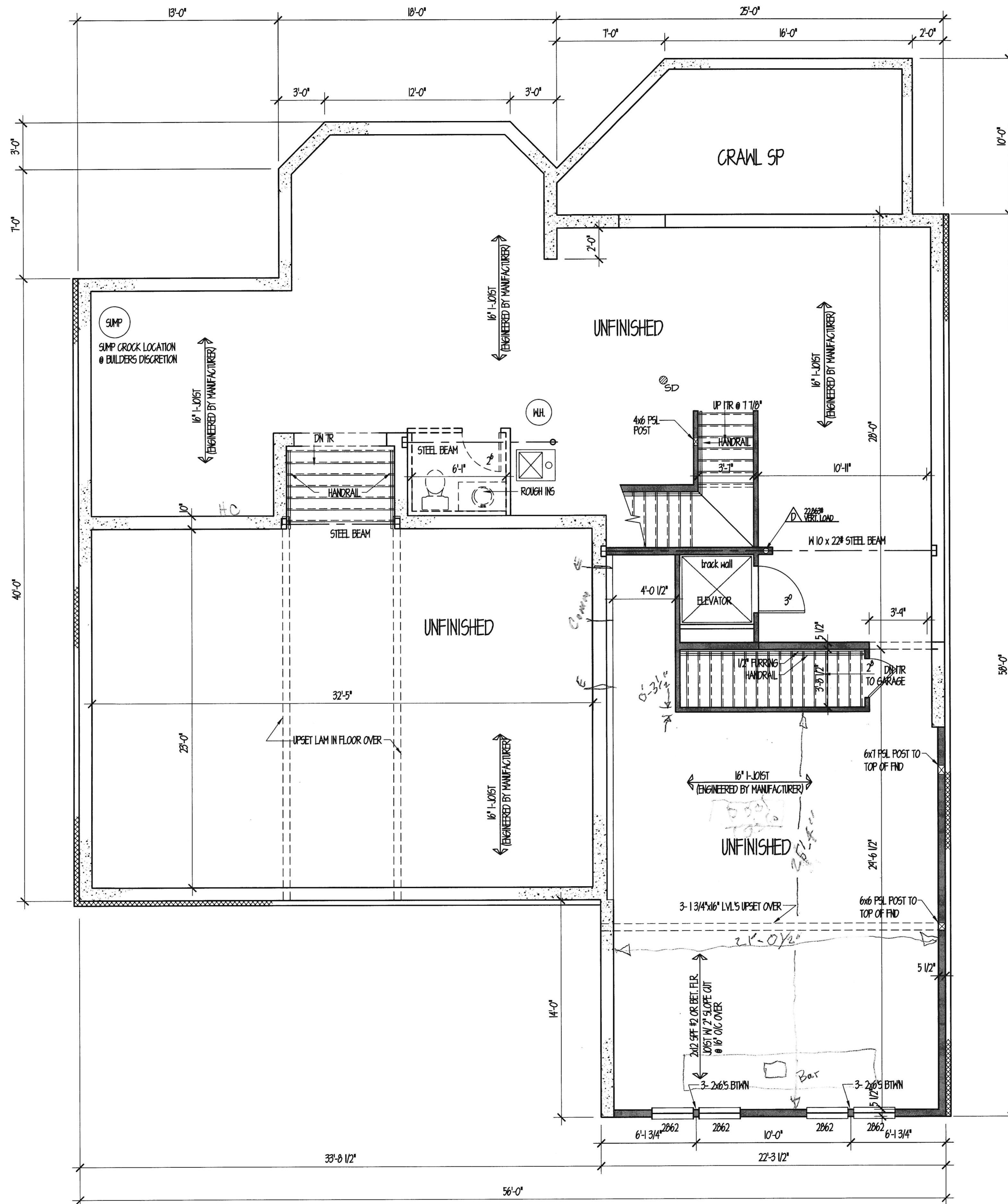
LOWER LEVEL PLAN 2826 S.F.
