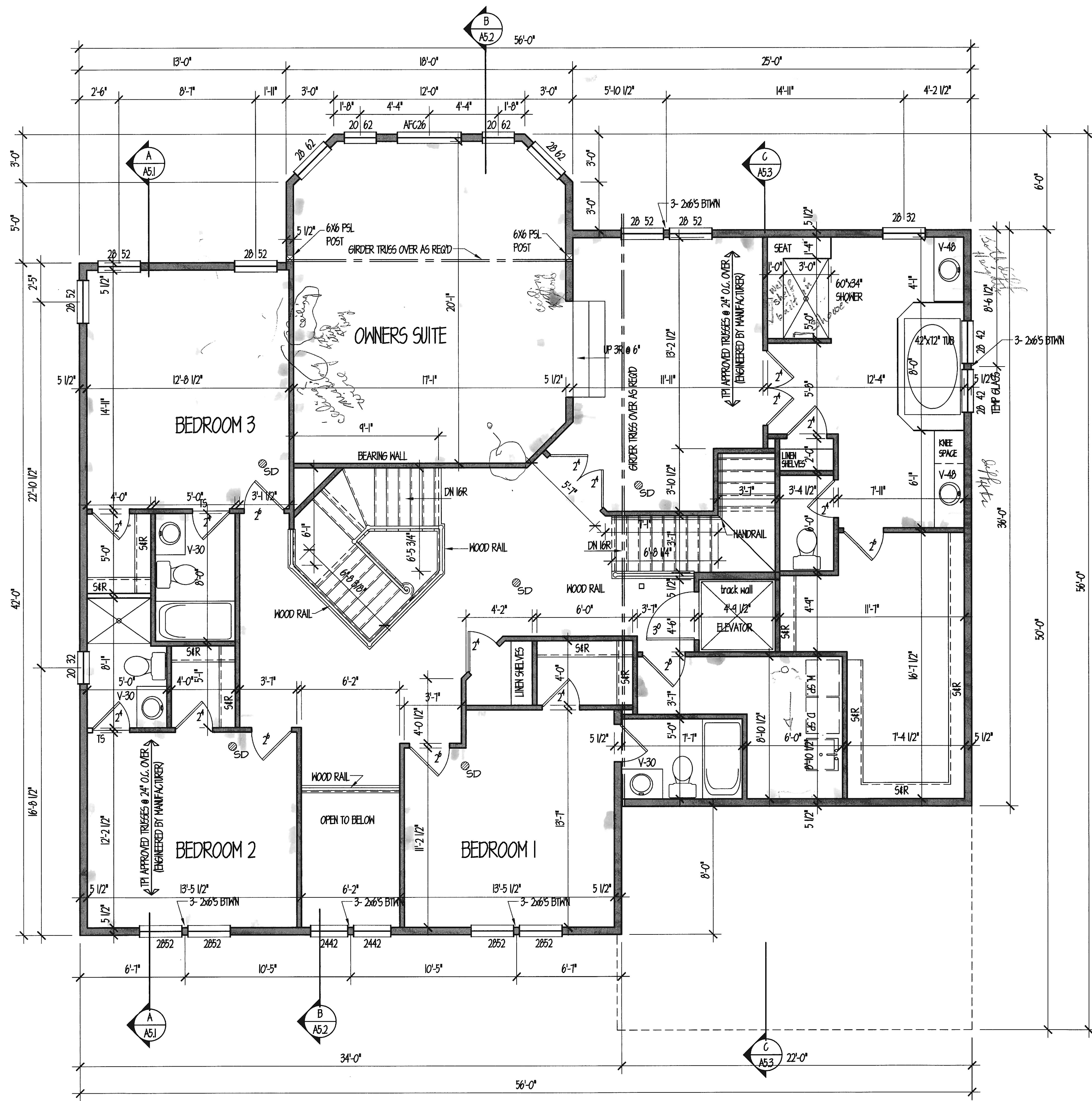
SECOND FLOOR PLAN 2360 S.F.
