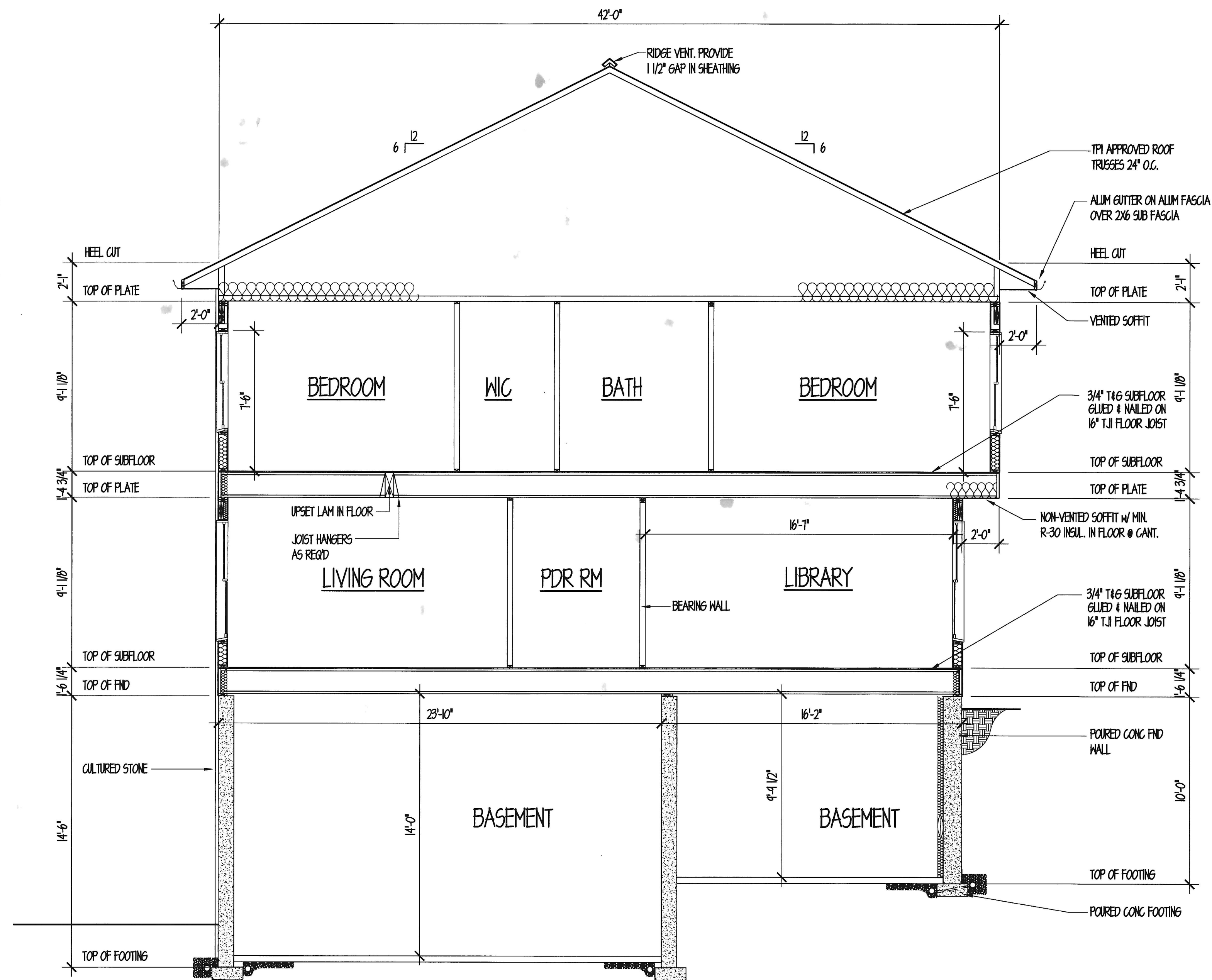
A A5.1 CROSS SECTION
