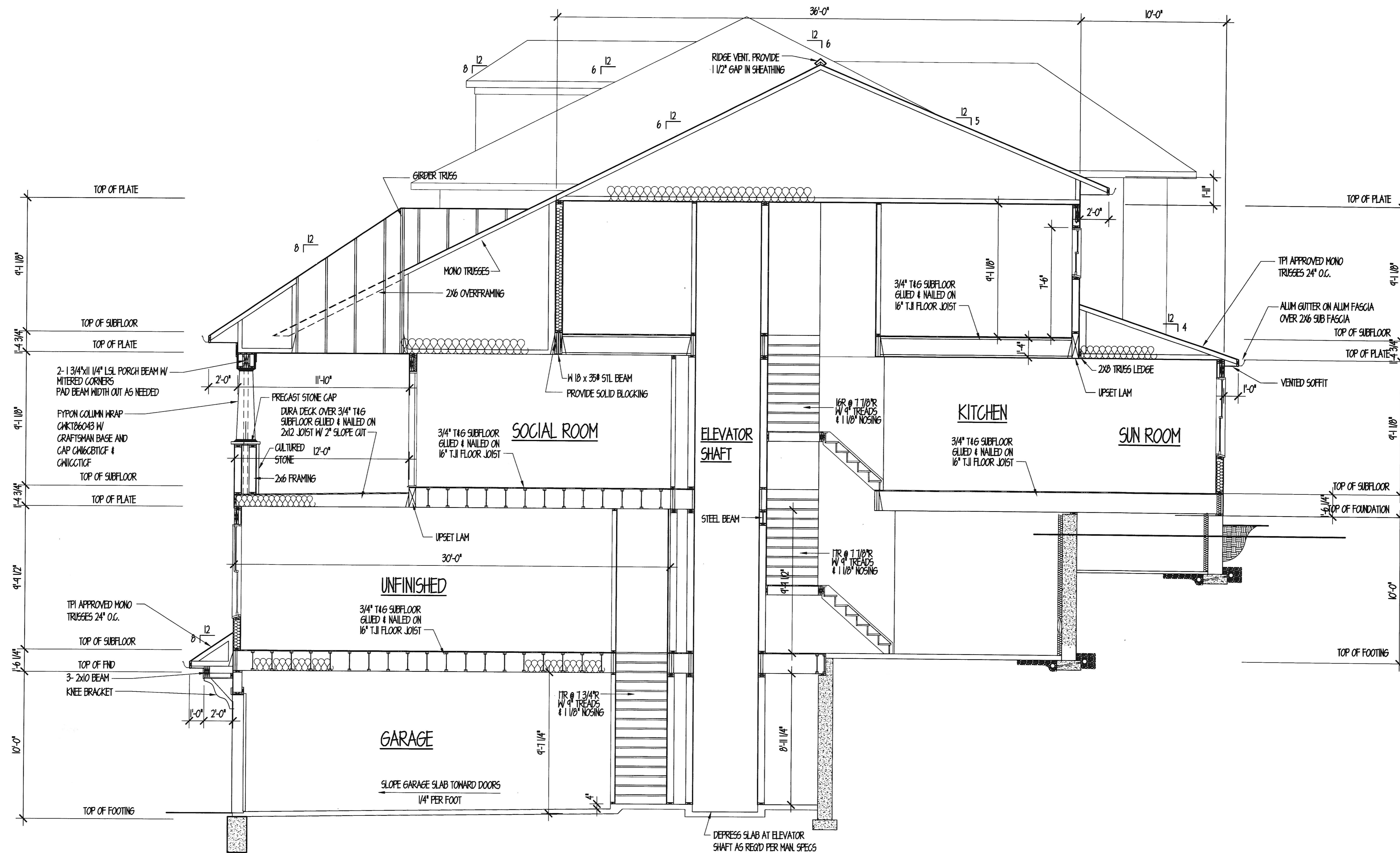
6 CROSS SECTION A5.3
