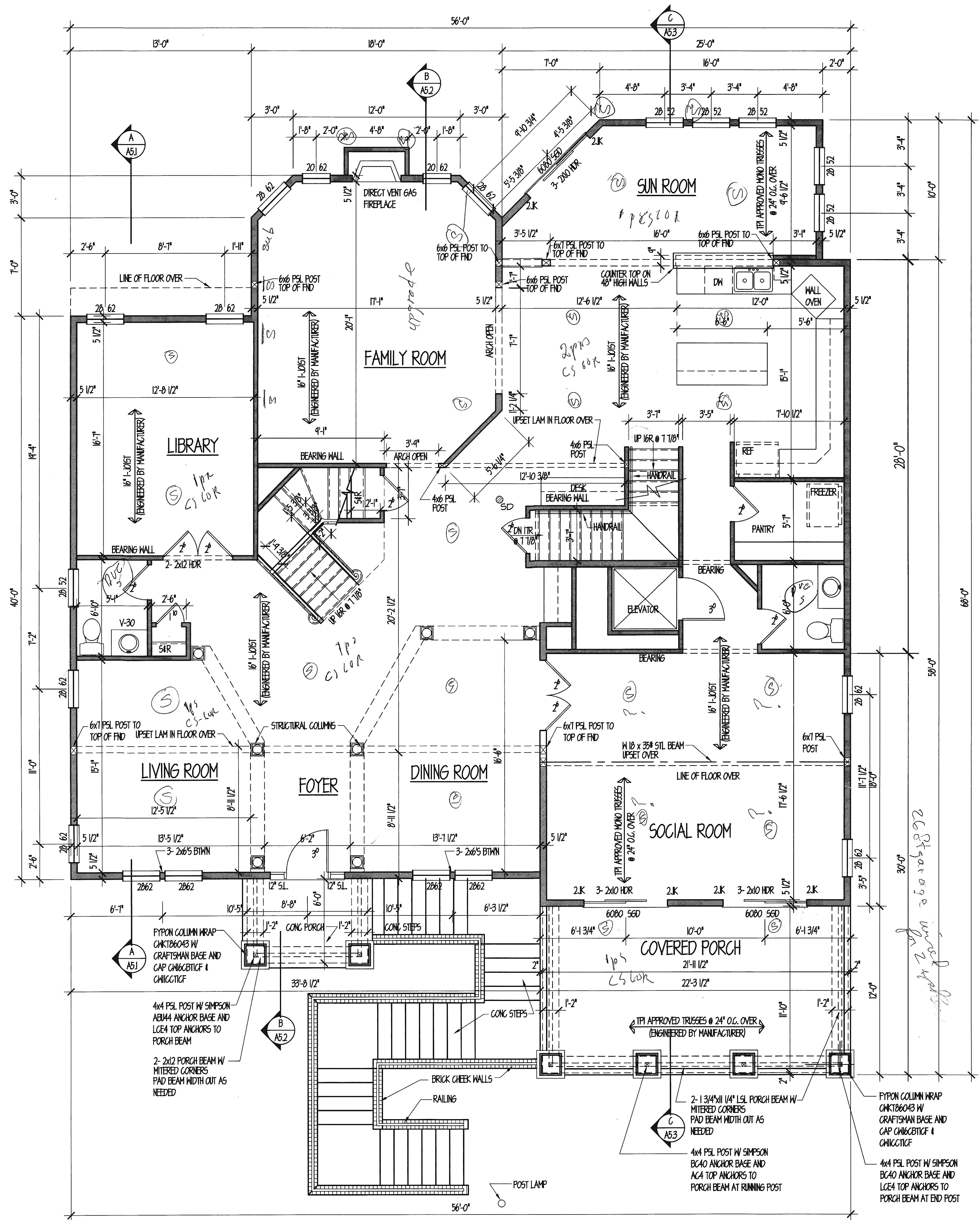
FIRST FLOOR PLAN 2,761 S.F.
