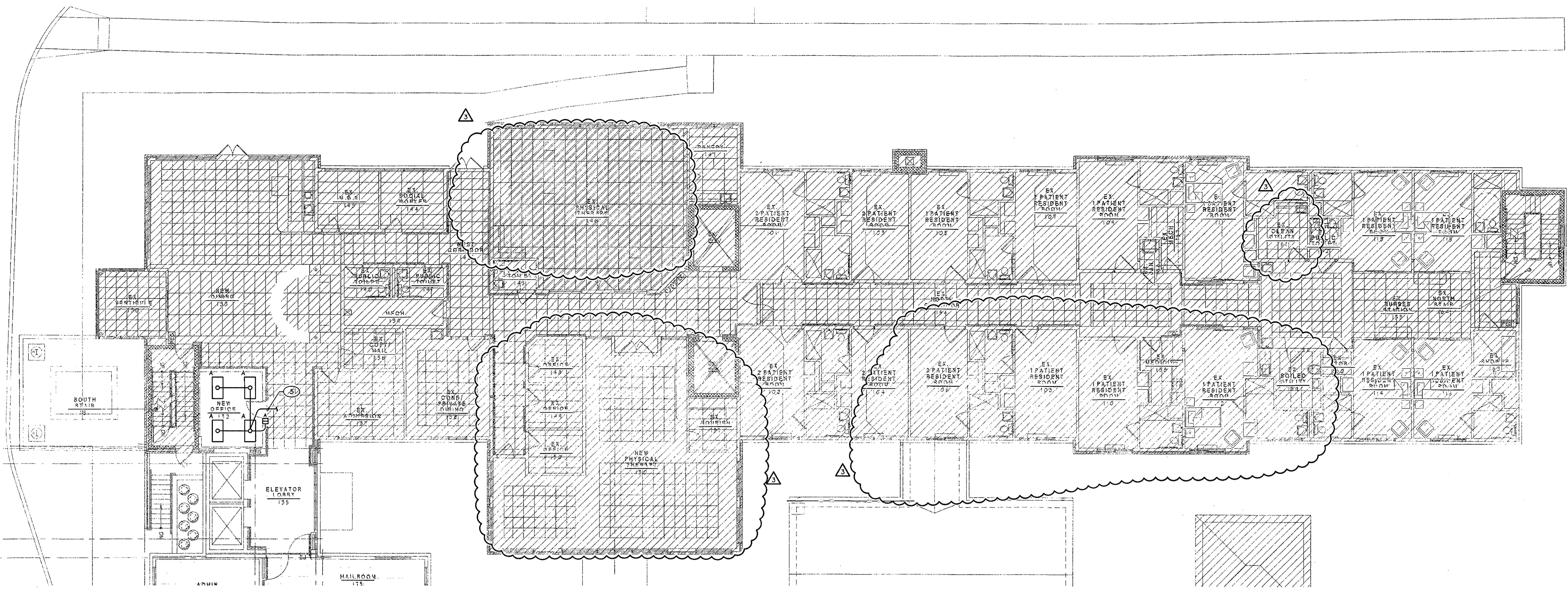
FIRST FLOOR PLAN - LIGHTING SCALE: 1/8" = 1'-0" 0' 2' 4' 8' 16'
