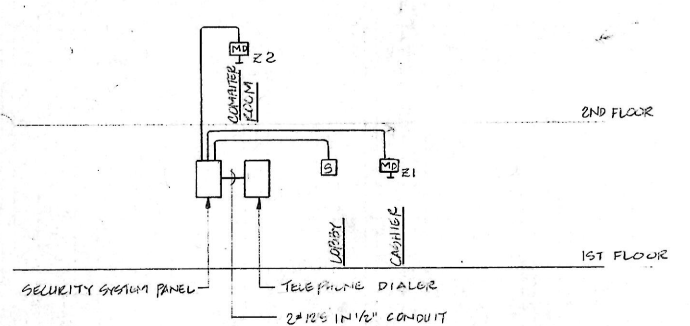
SECURITY SYSTEM RISER DIAGRAM SCALE: NONE
