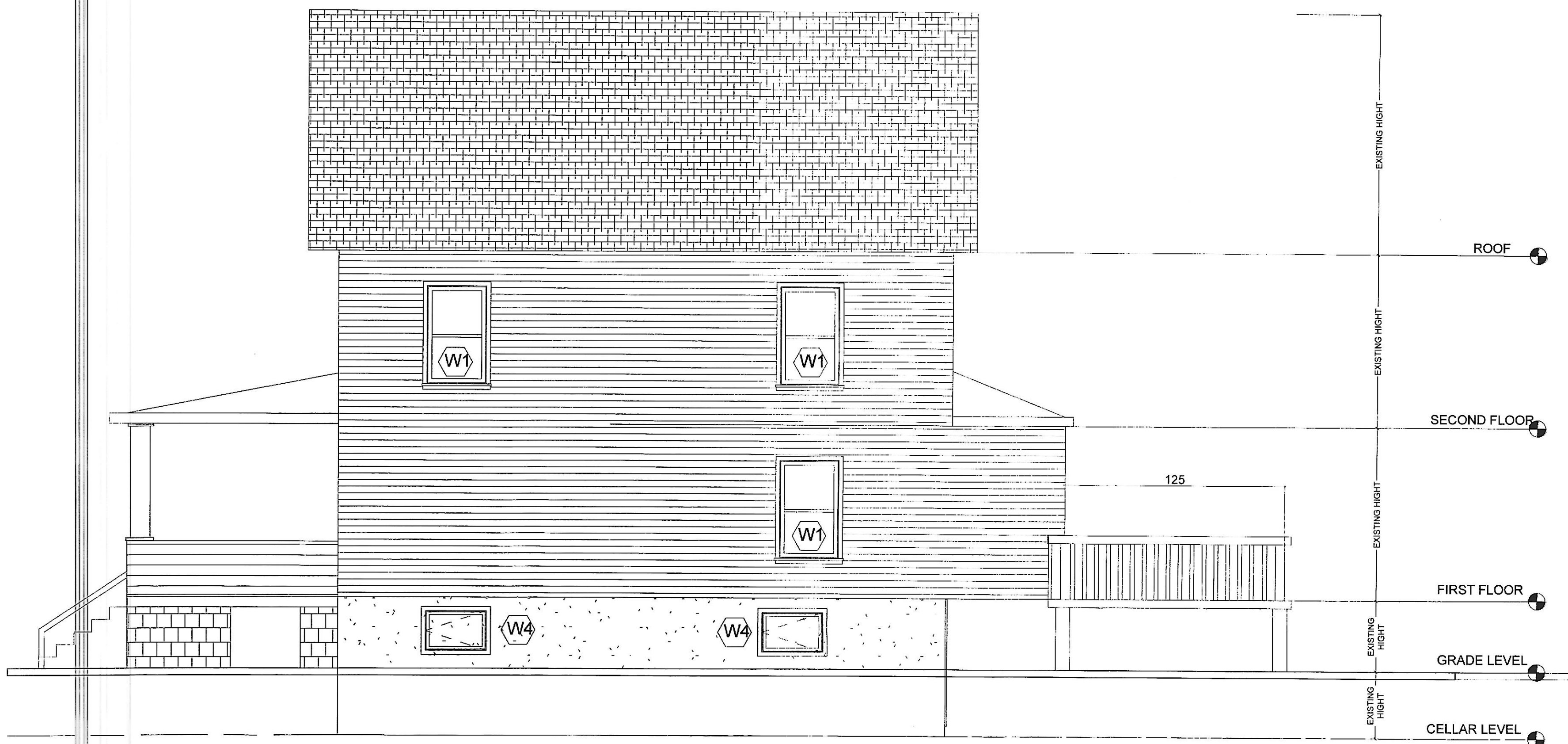
PROPOSED NORTH (LEFT) VIEW SCALE = 1/4"=1'-0"
