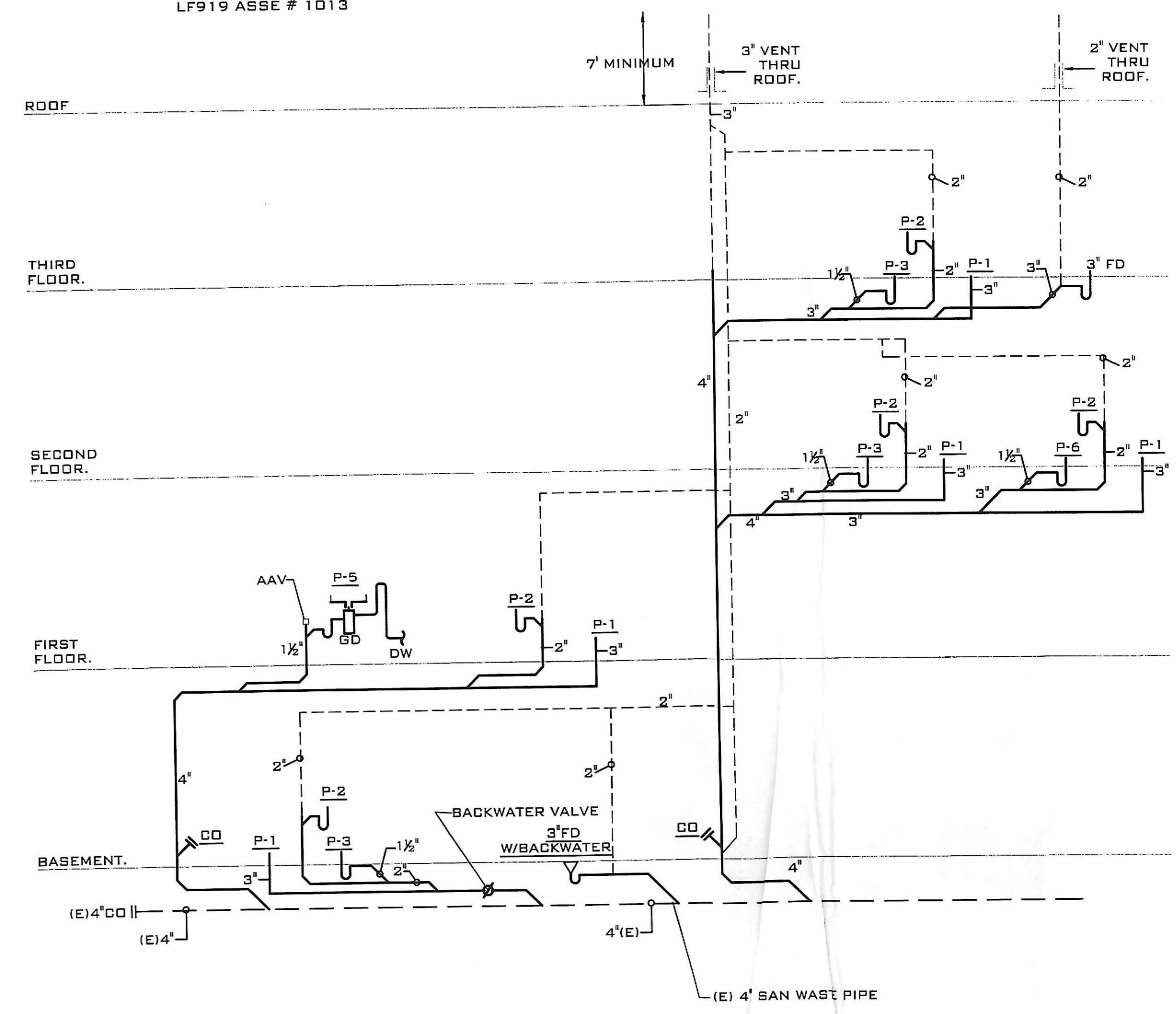
SANITARY RISER DIAGRAM NOT TO SCALE
