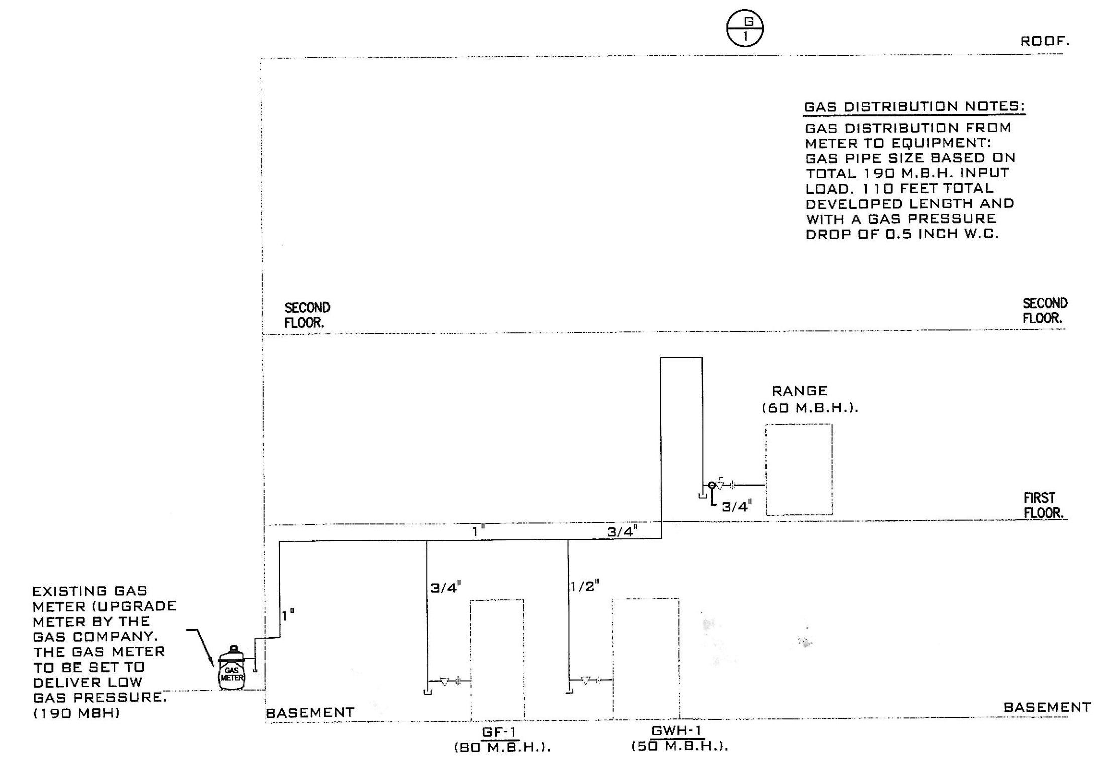
GAS RISER DIAGRAM NOT TO SCALE
