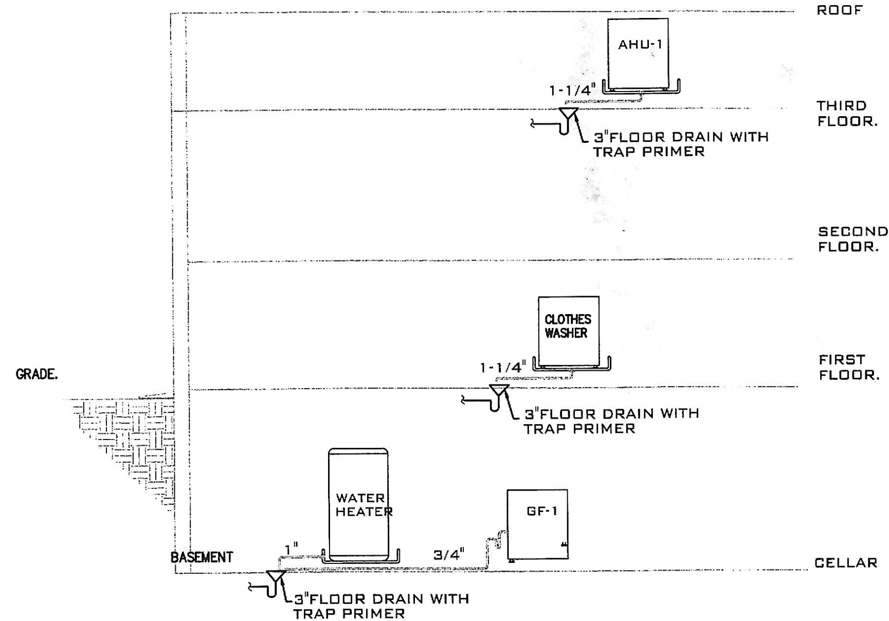
CONDENSATED AND SAFETY DRAINS RISER DIAGRAM NOT TO SCALE
