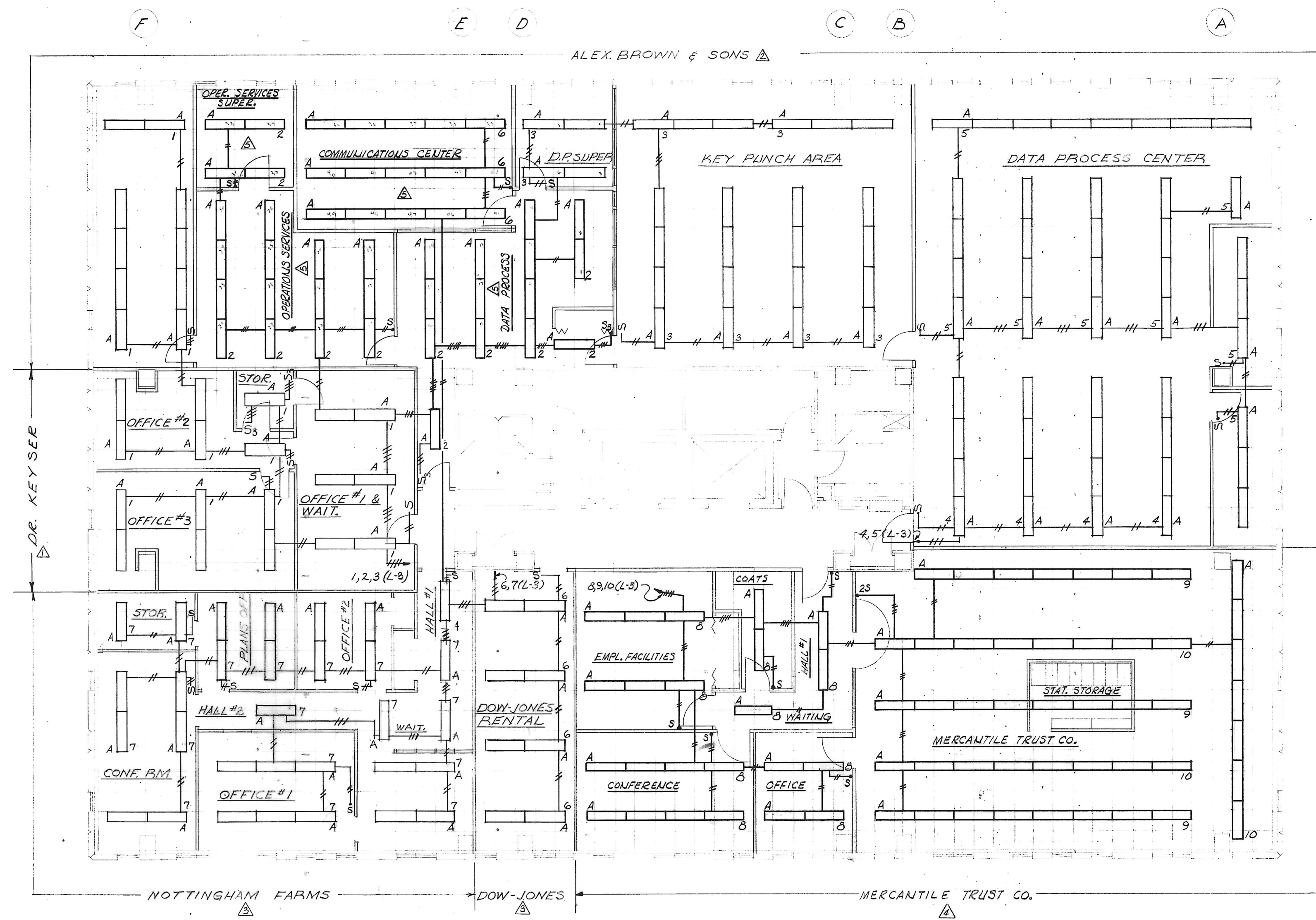
THIRD FLOOR PLAN (AT CEILING) Scale: 1/8" = 1'-0"
