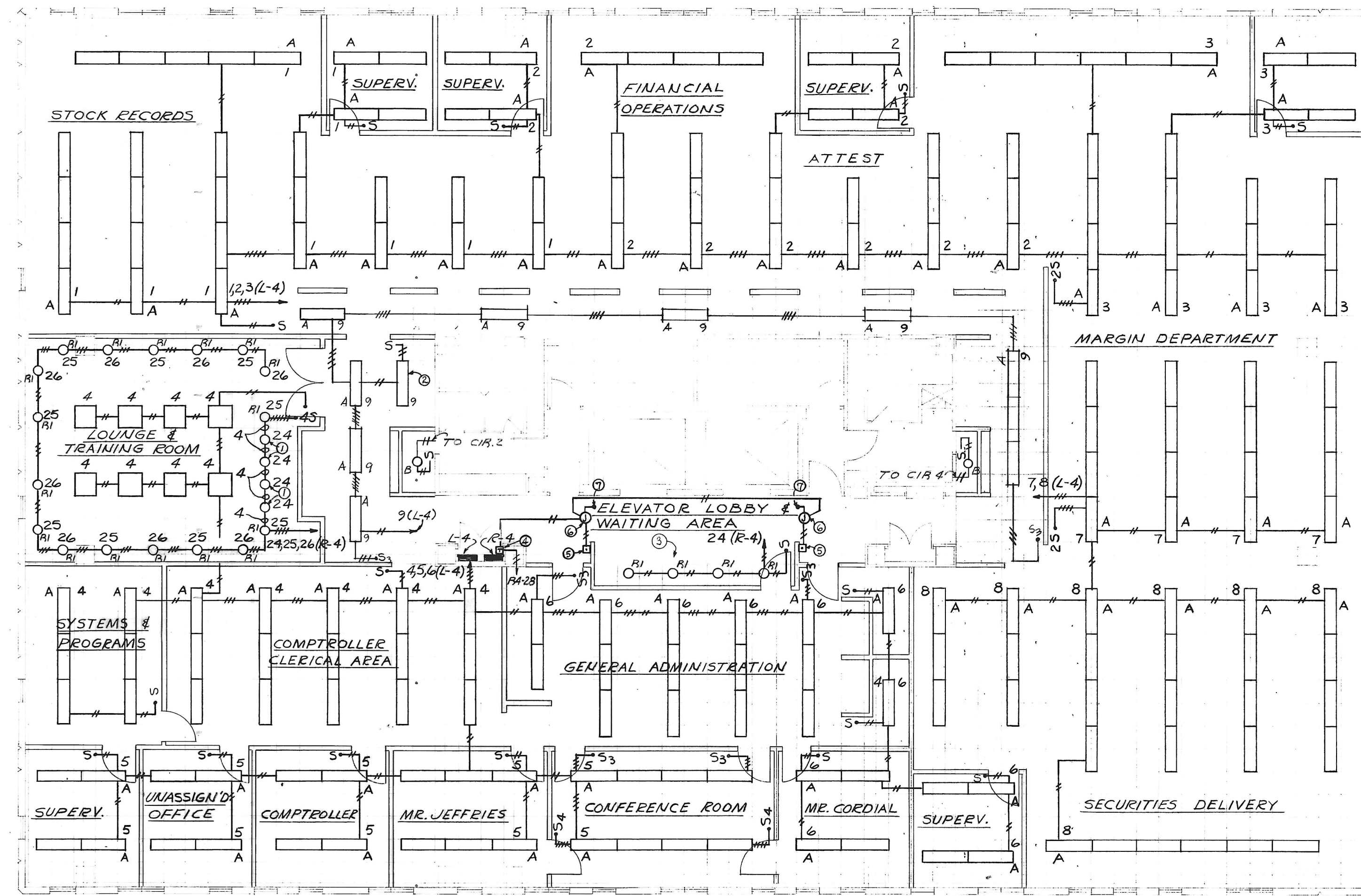
ALEX. BROWN & SONS Δ FOURTH FLOOR PLAN (AT CEILING) Scale: 1/8" = 1'-0"
