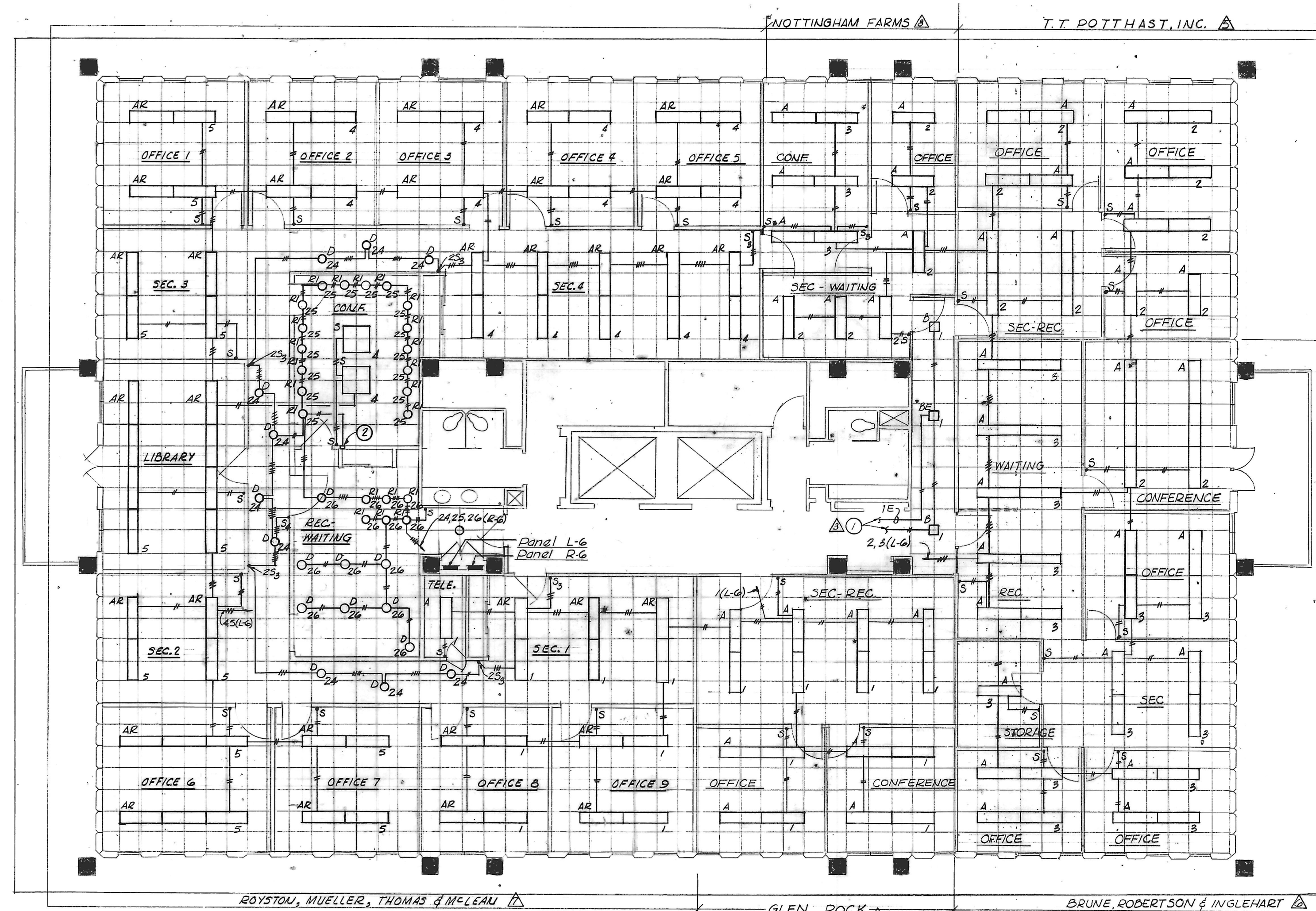
SIXTH FLOOR PLAN (AT CEILING) Scale: 1/8" = 1'-0"
