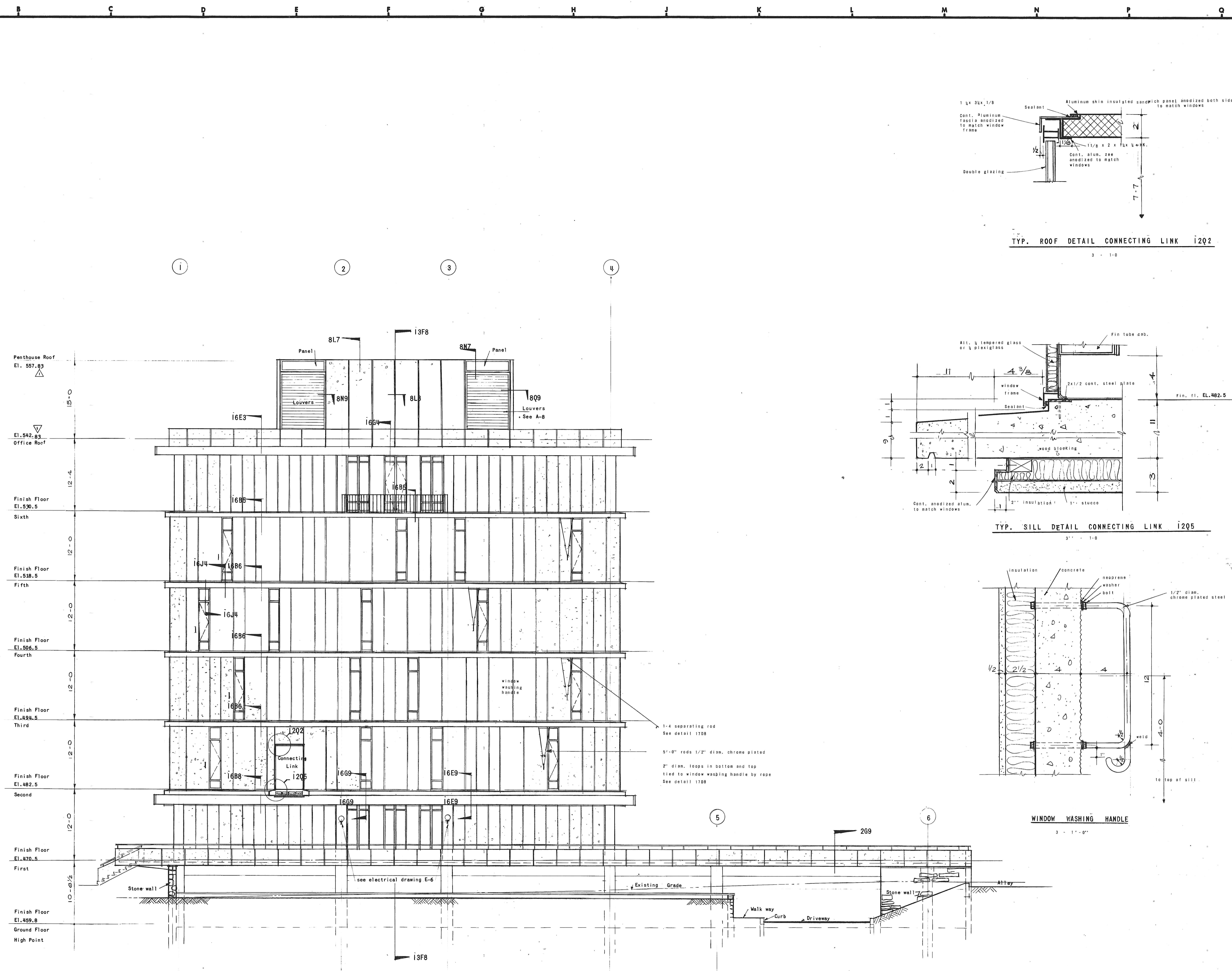
EAST ELEVATION 12M8 1/8 - 1-0
