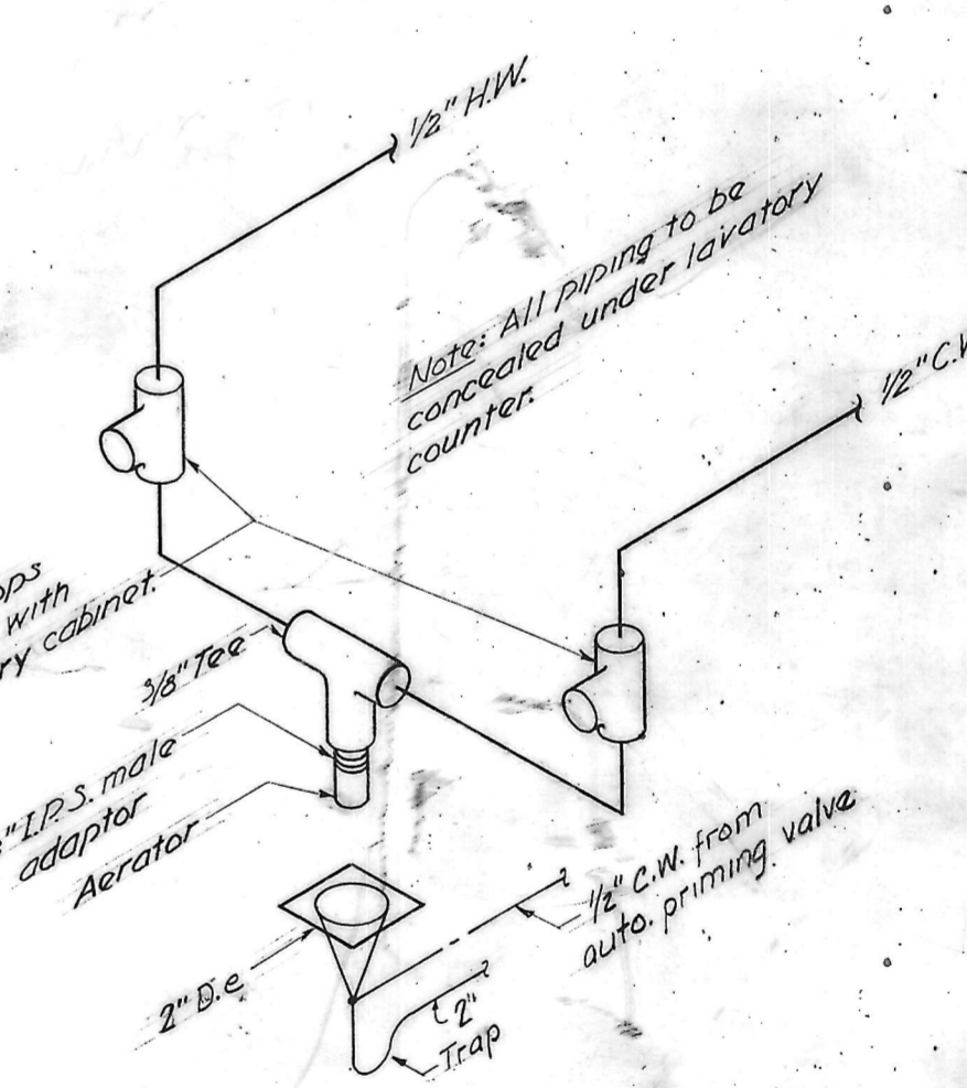
DETAIL OF WATER MIXER (P5) No Scale
