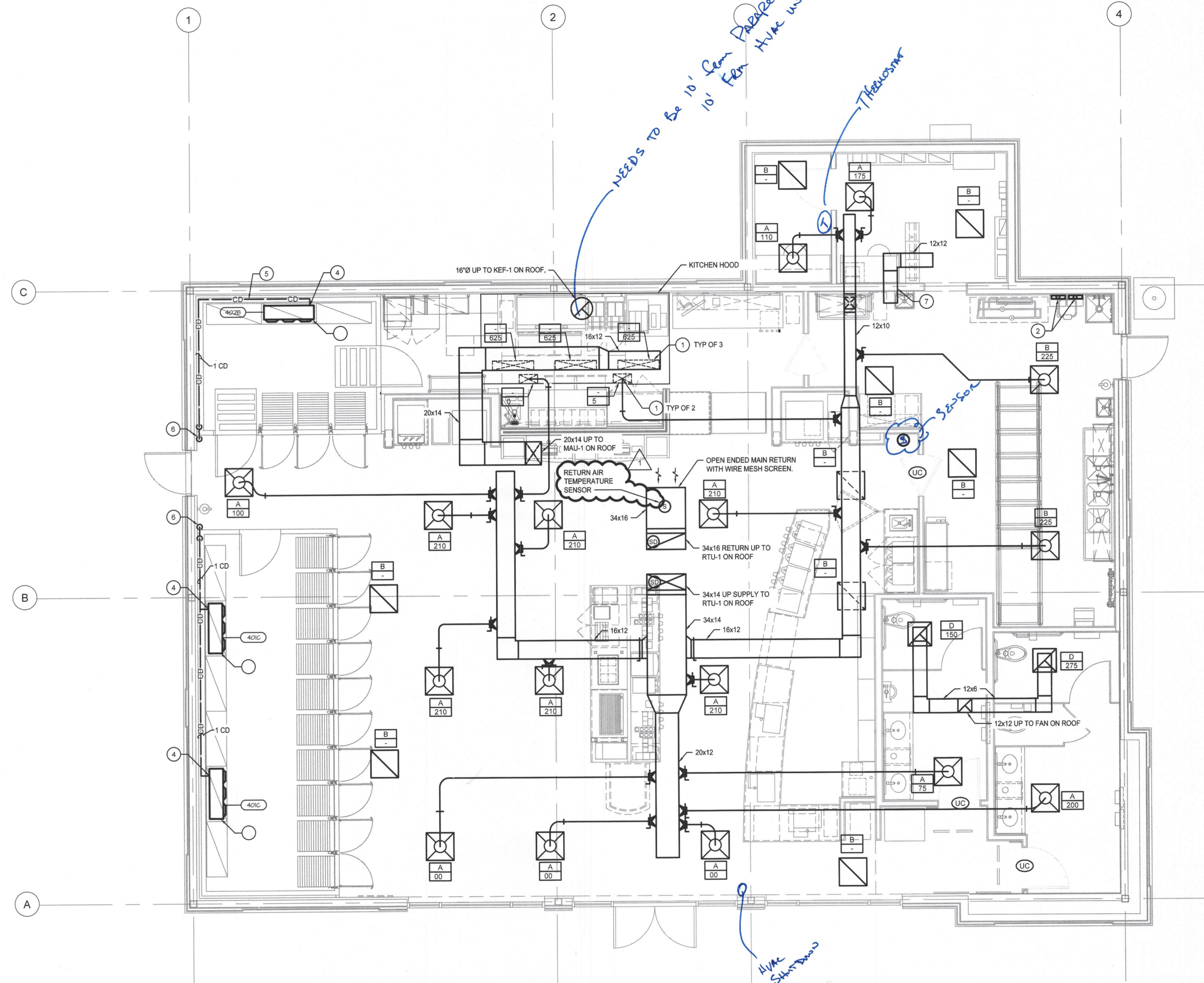
1 FLOOR PLAN - MECHANICAL S 1/4" = 1'-0"
