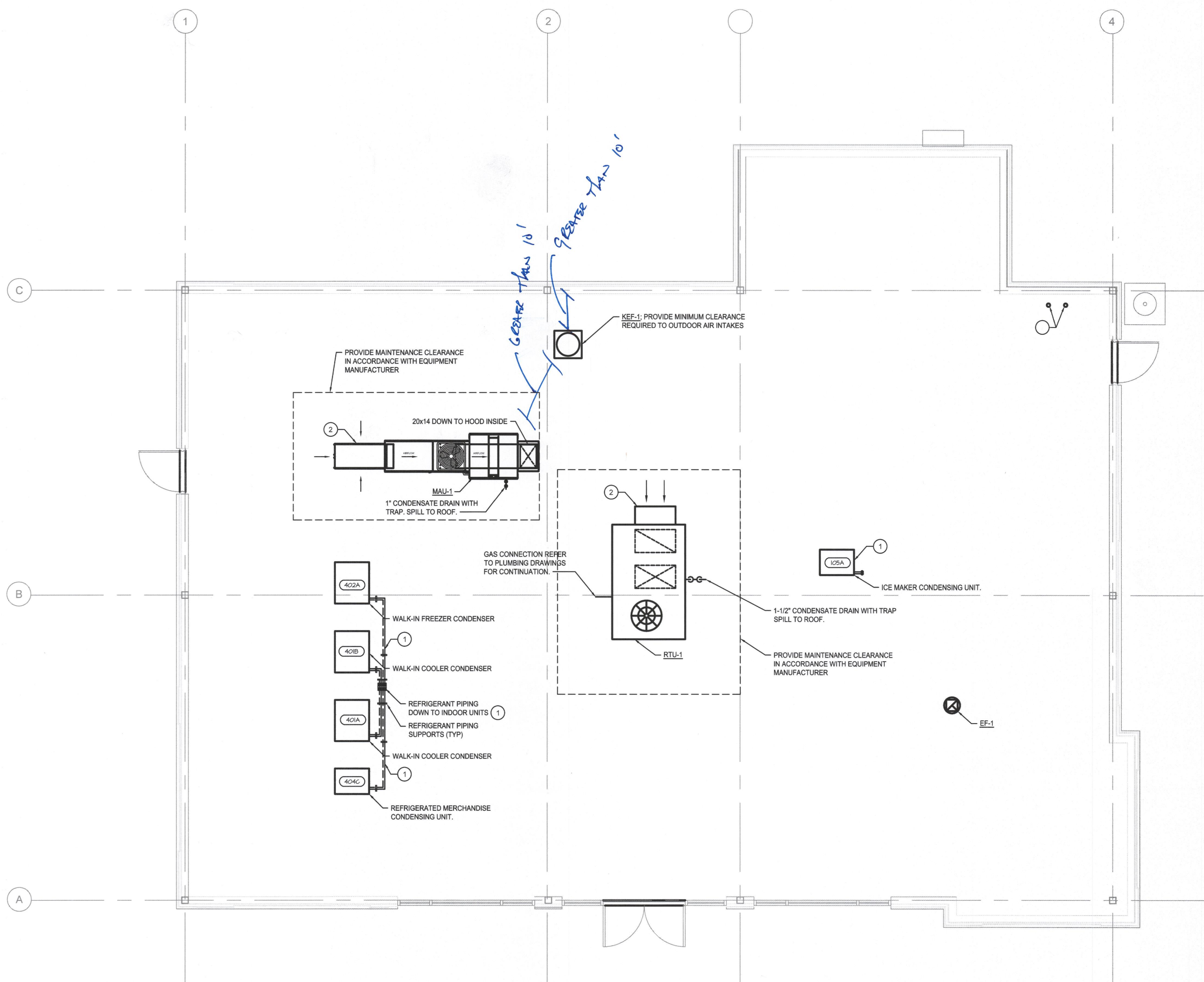
1 ROOF PLAN - MECHANICAL S 1/4" 1'-0"
