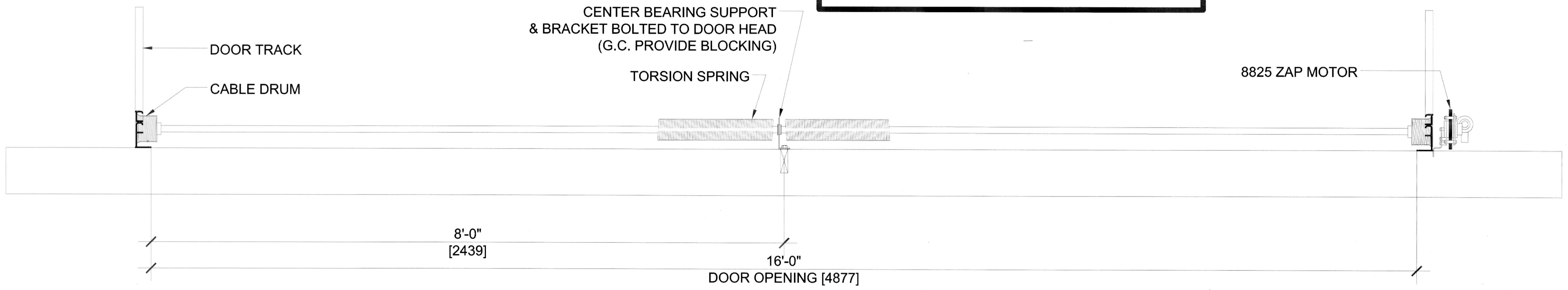
01 DOOR PLAN BELOW HEAD A SCALE: 3/4" = 1'
