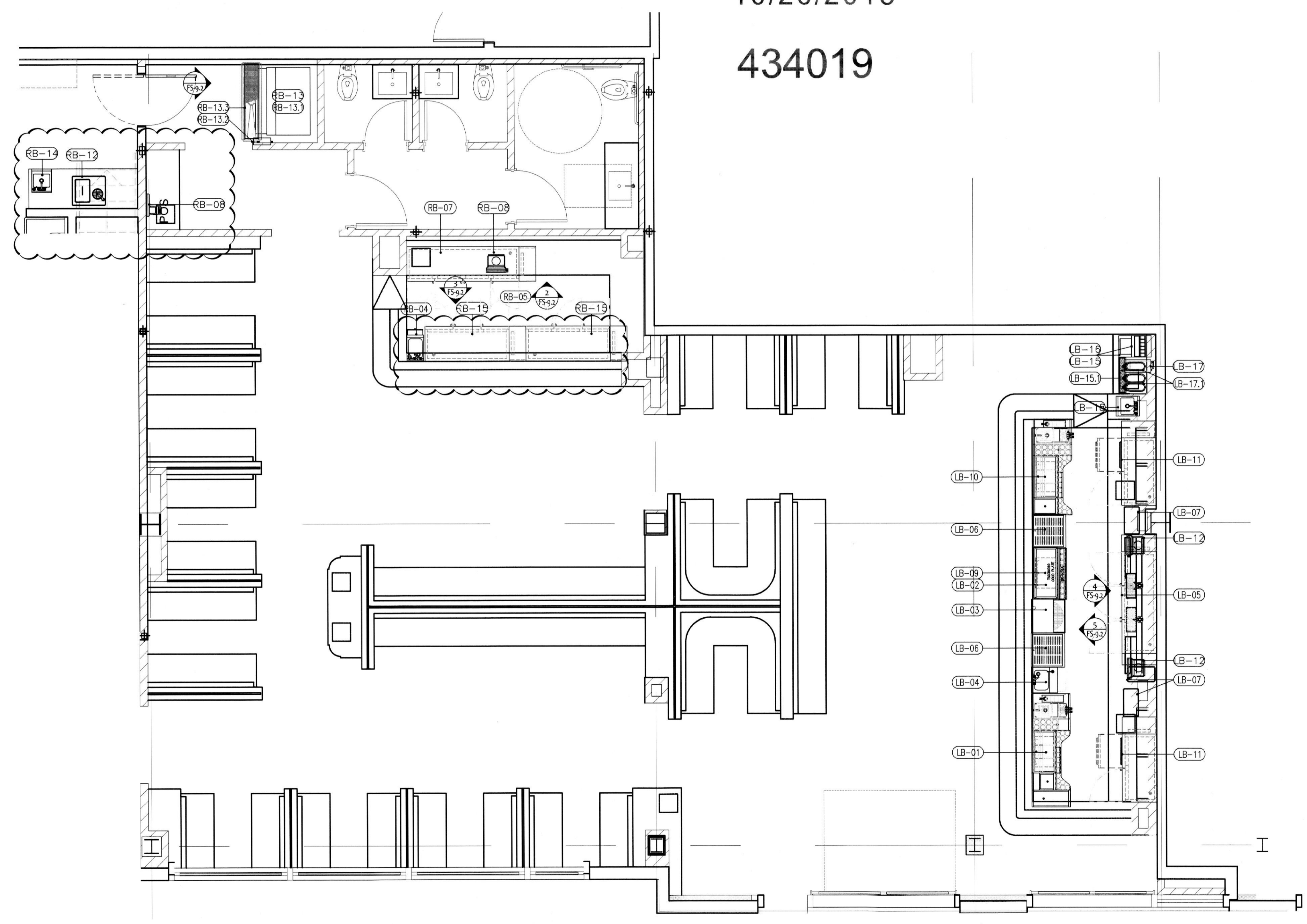
1 LOCH BAR EQUIPMENT LAYOUT AND SCHEDULE SCALE: 1/4" = 1' 0"
