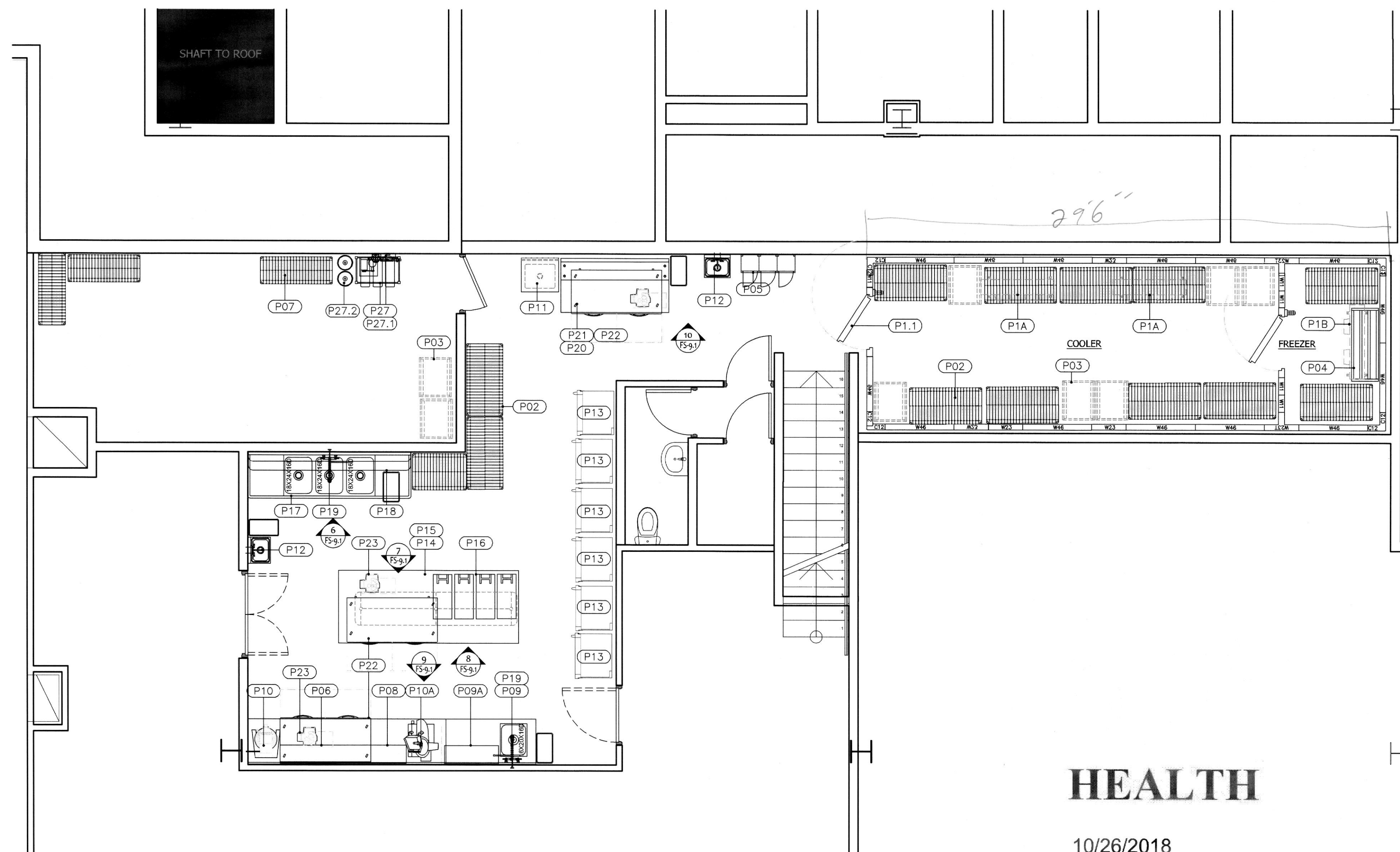
1 MEZZANINE EQUIPMENT LAYOUT AND SCHEDULE SCALE: 1/4" = 1' 0"
