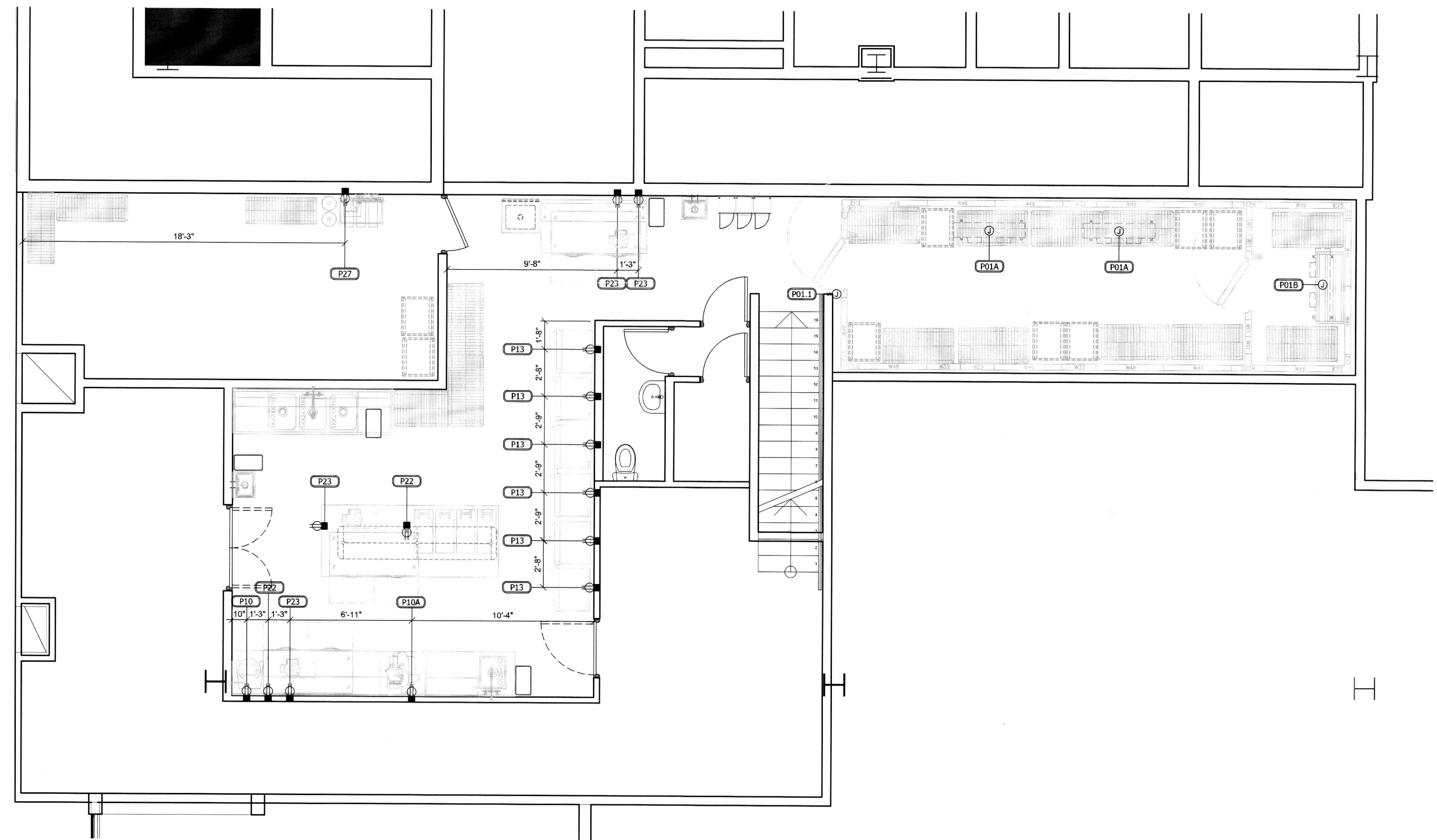
1 MEZZANINE ELECTRICAL ROUGH-IN PLAN & SCHEDULE Scale: 1/4" = 1' 0"
