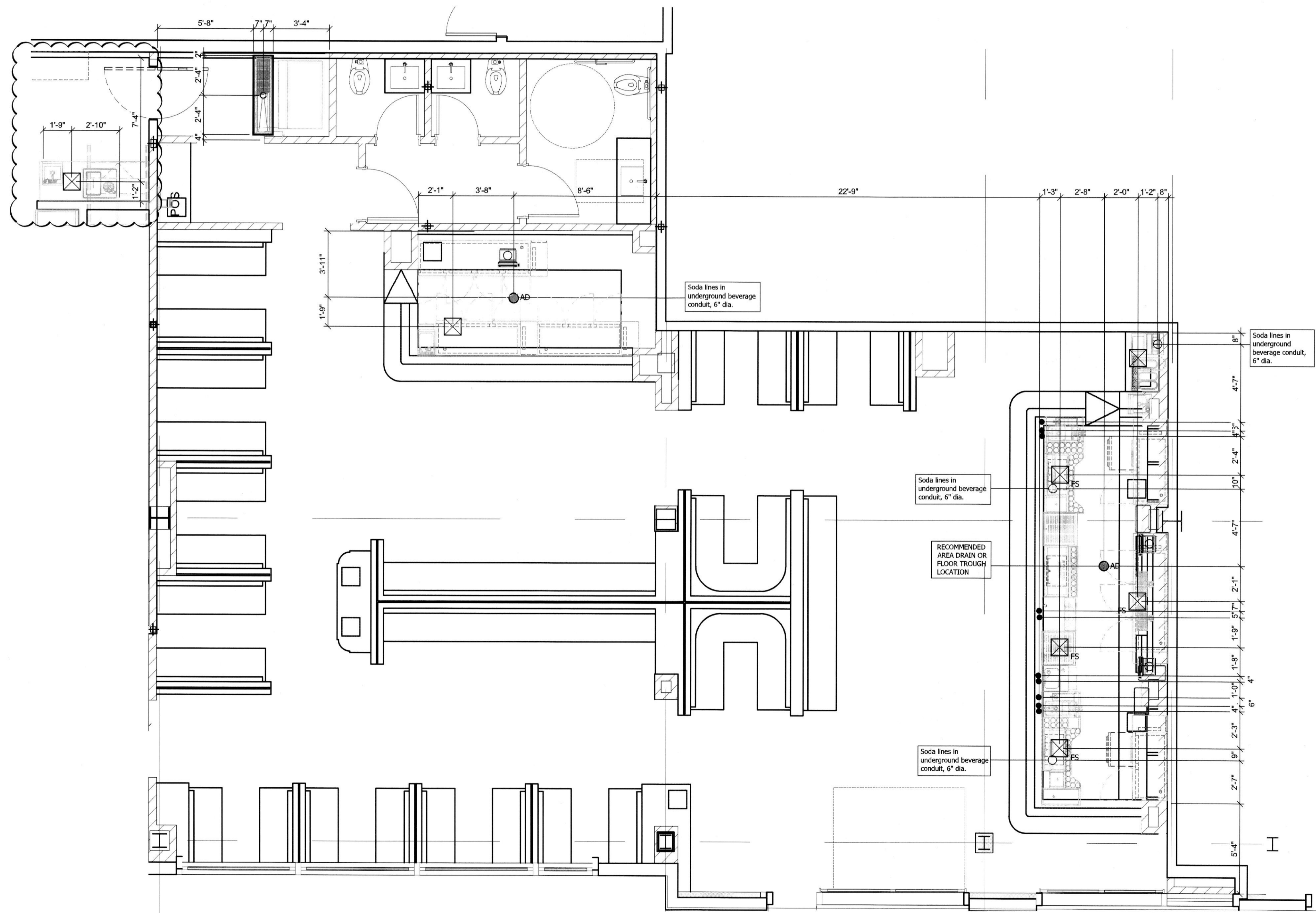
1 LOSH BAR SLAB PENETRATIONS PLAN
