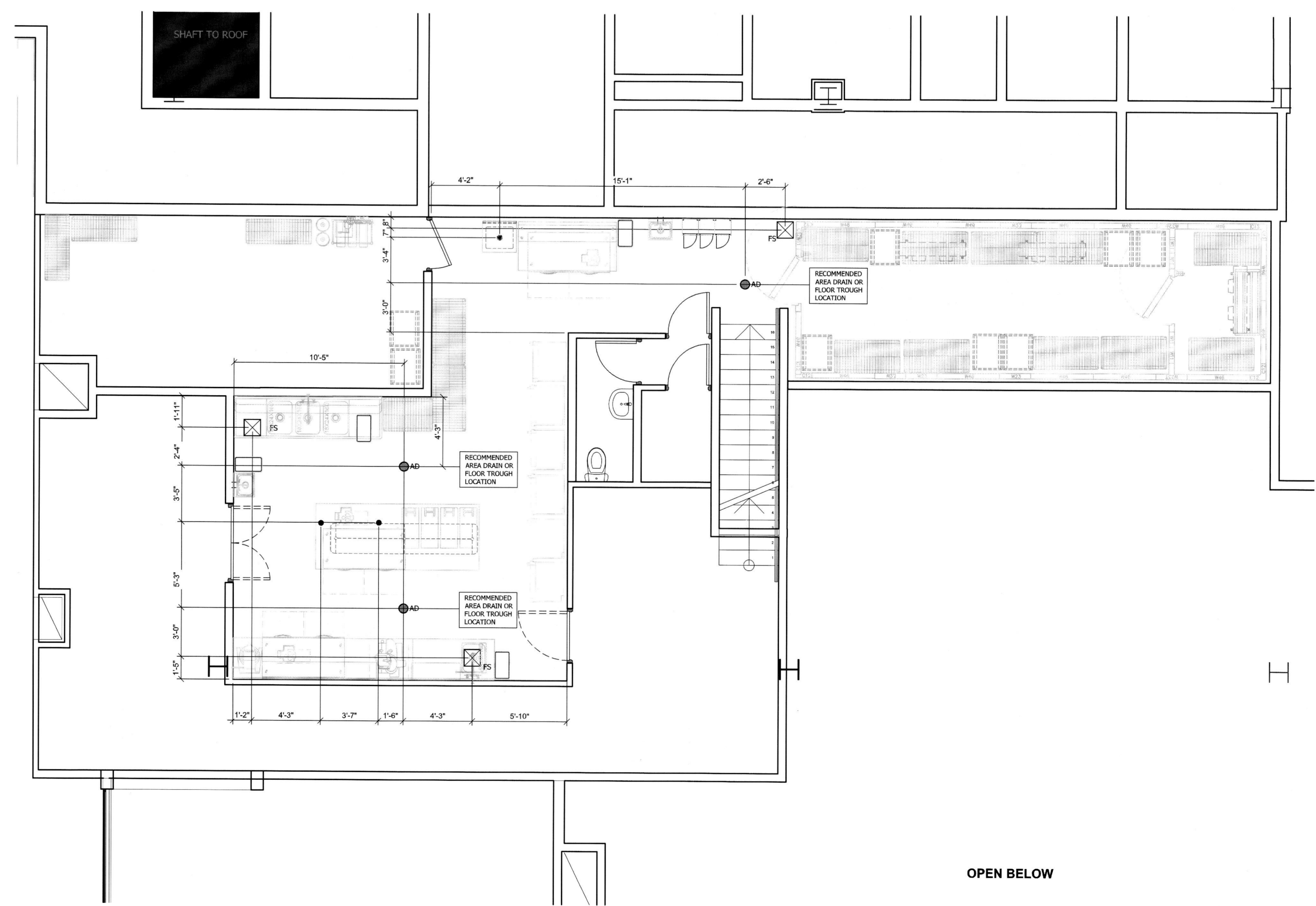
1 SLAB PENETRATIONS PLAN Scale: 1/4" = 1' 0"
