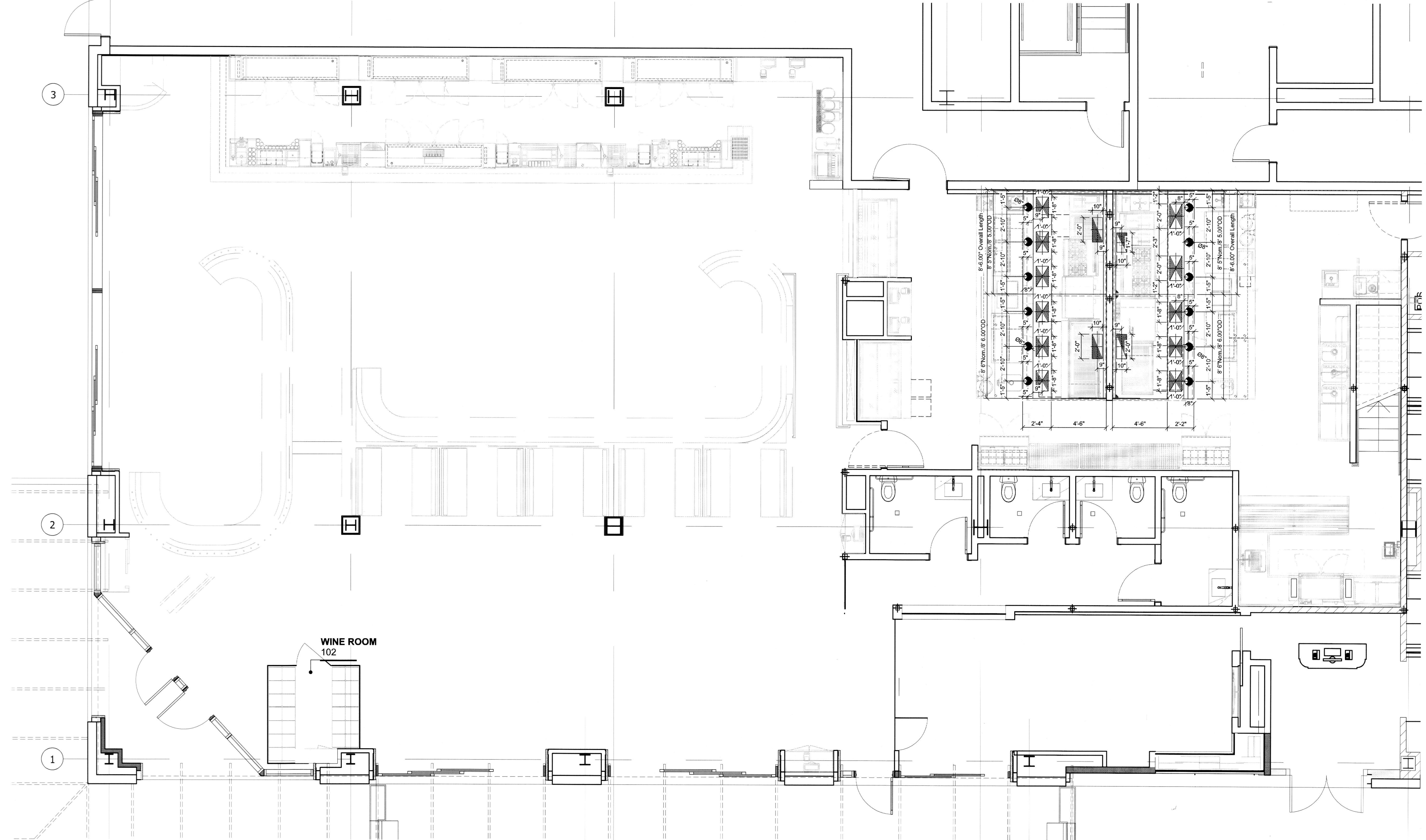
1 OUZO KITCHEN AND BAR VENTILATION PLAN Scale: 1/4" = 1' 0"
