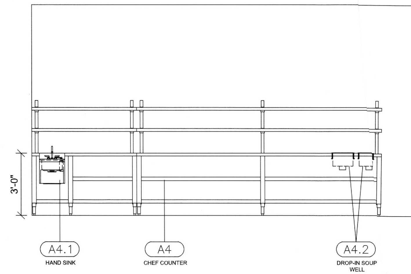
5 CHEF COUNTER - EXPO SIDE SCALE: 3/8" = 1'-0"
