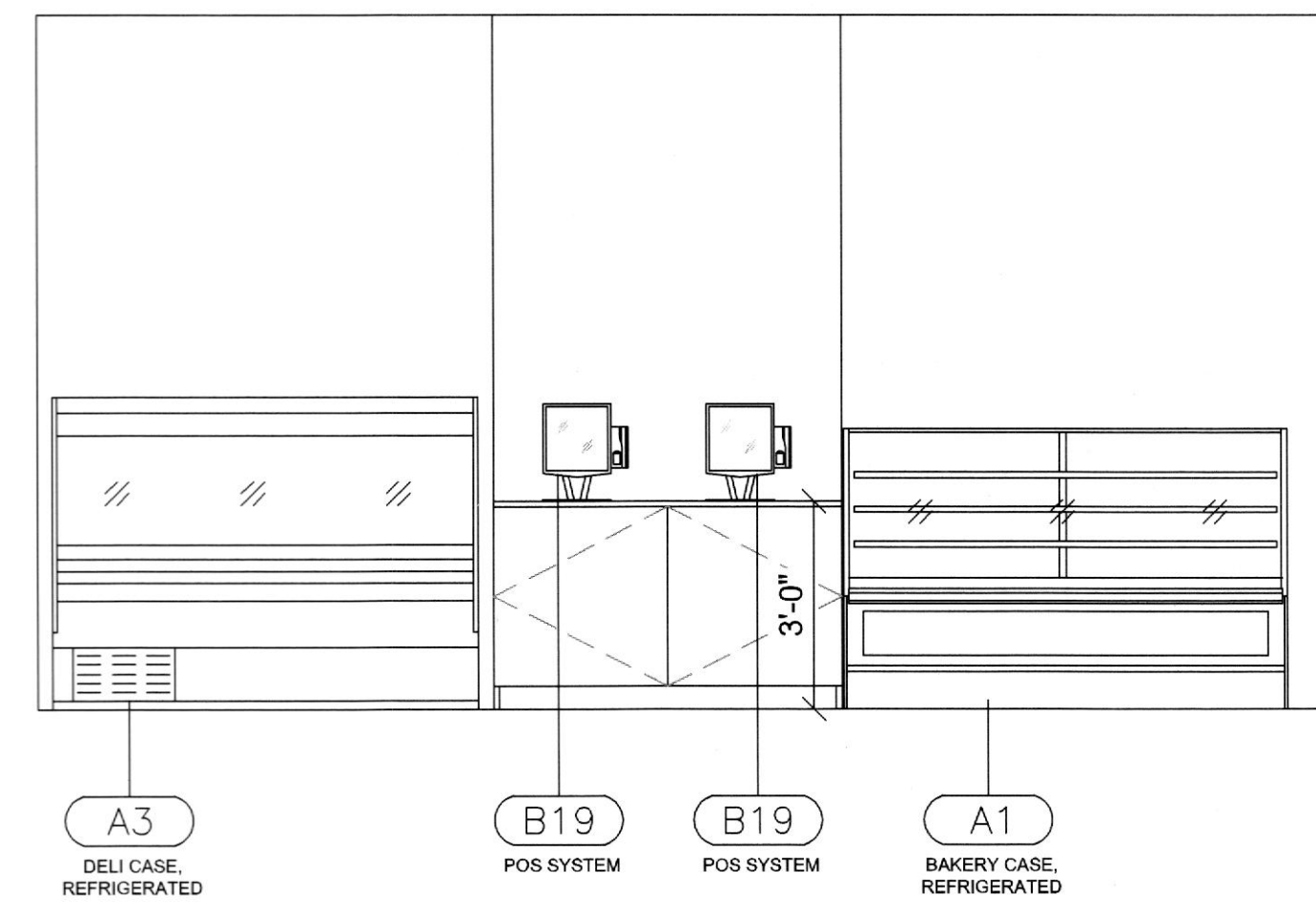
4 FRONT COUNTER SCALE: 3/8" = 1'-0"
