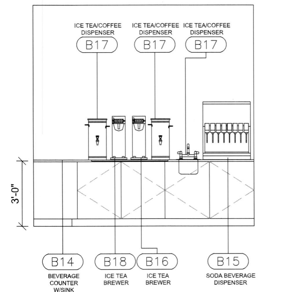
3 BACKBAR BEVERAGE STATION SCALE: 3/8" = 1'-0"
