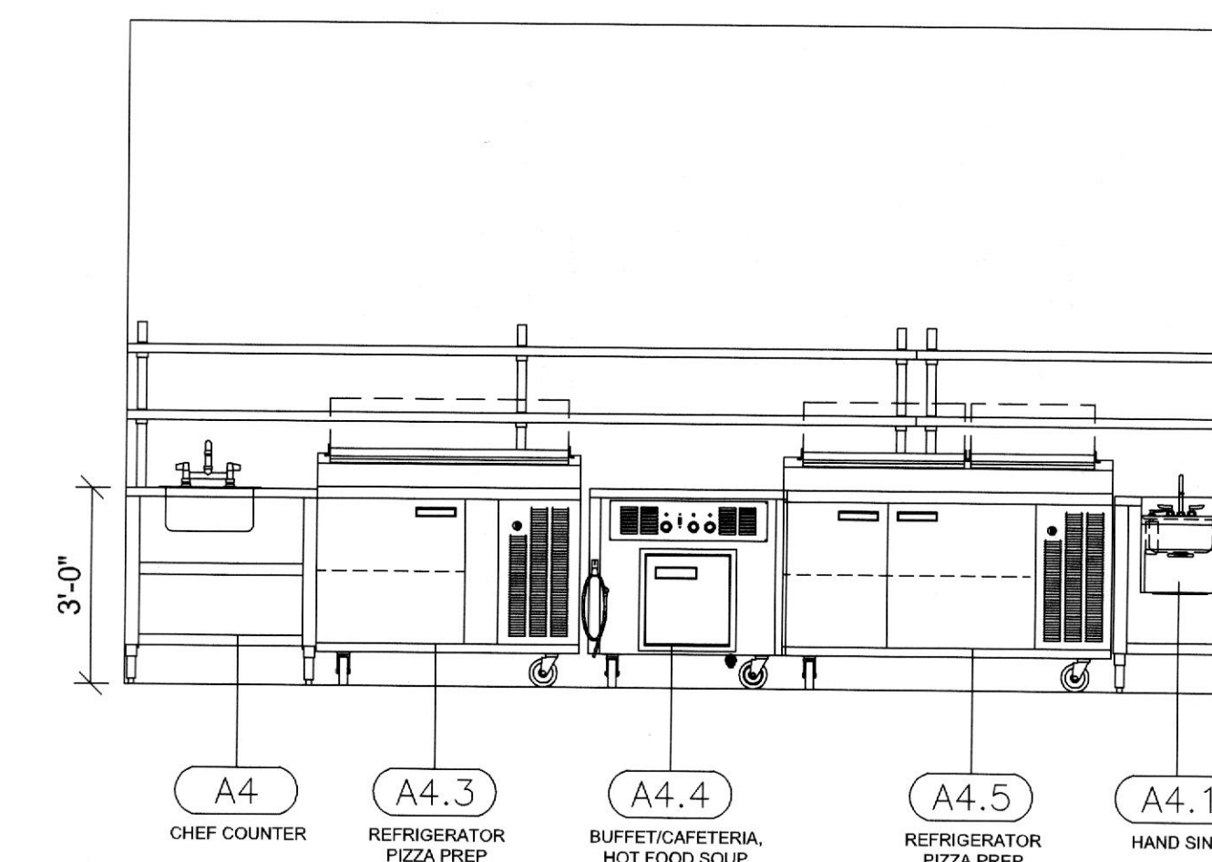
6 CHEF COUNTER SCALE: 3/8" = 1'-0"
