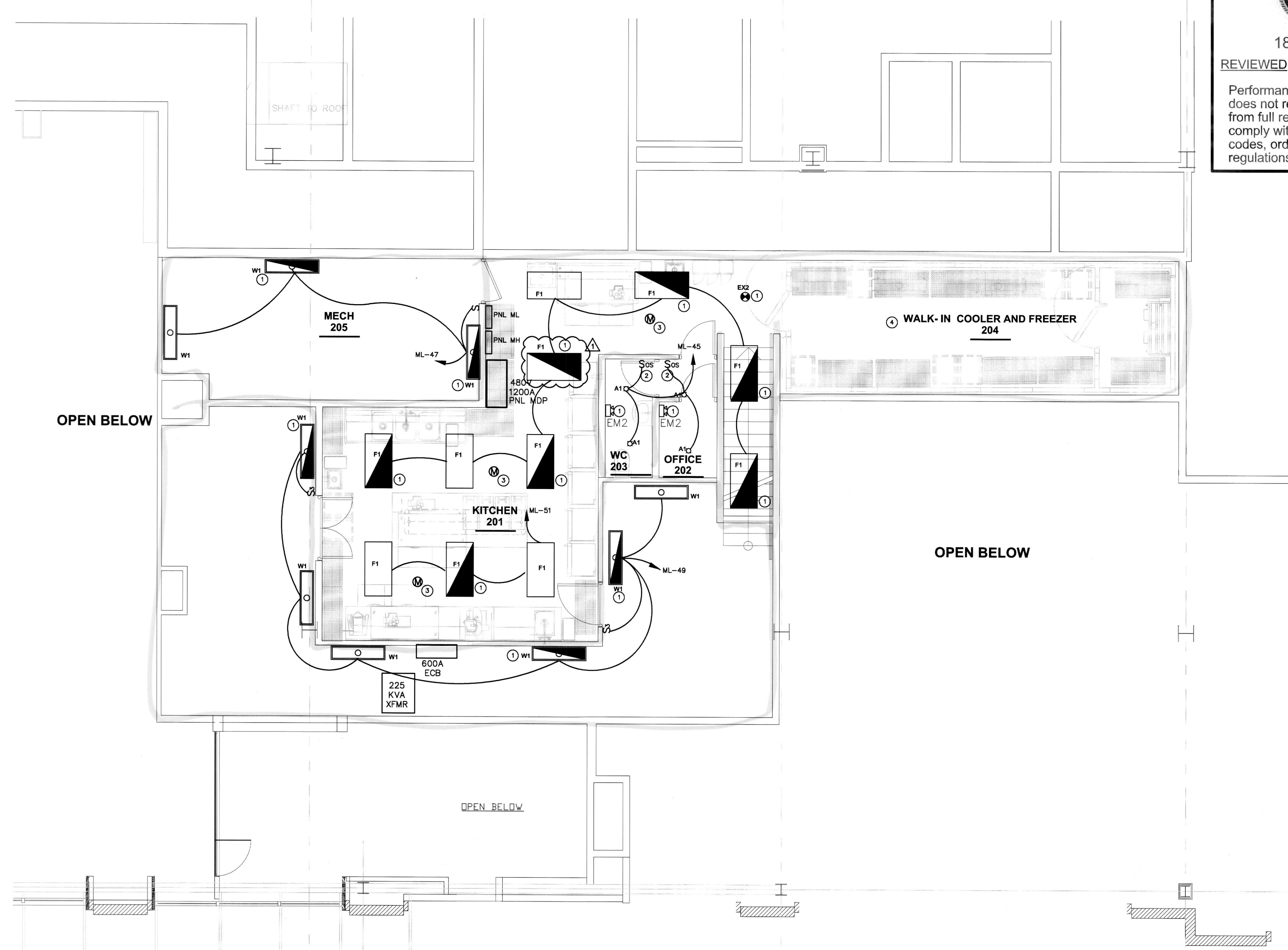
1 MEZZANINE LEVEL - LIGHTING PLAN SCALE: 1/4" = 1'-0"
