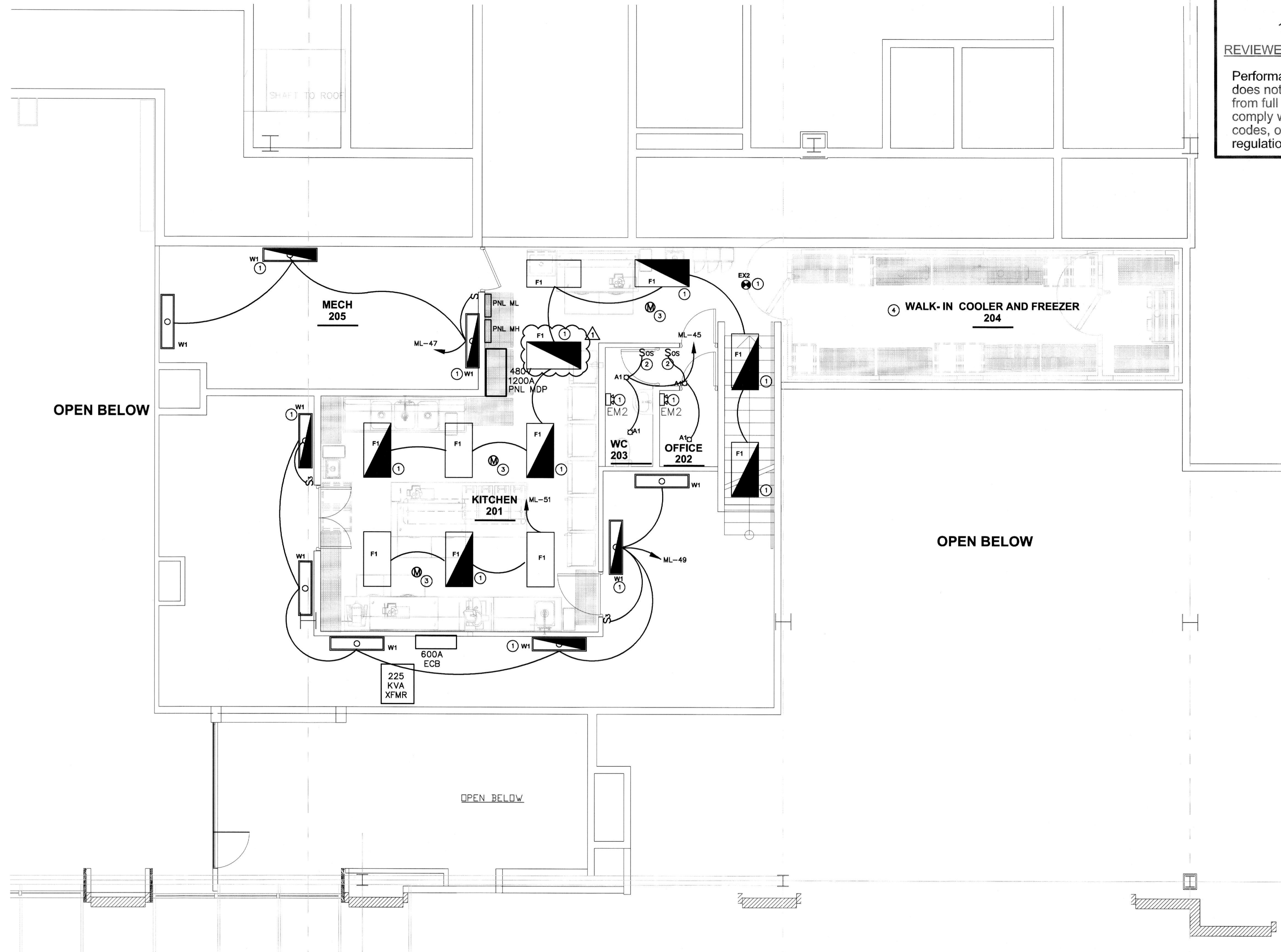
1 MEZZANINE LEVEL - LIGHTING PLAN E.07 SCALE: 1/4" = 1'-0"
