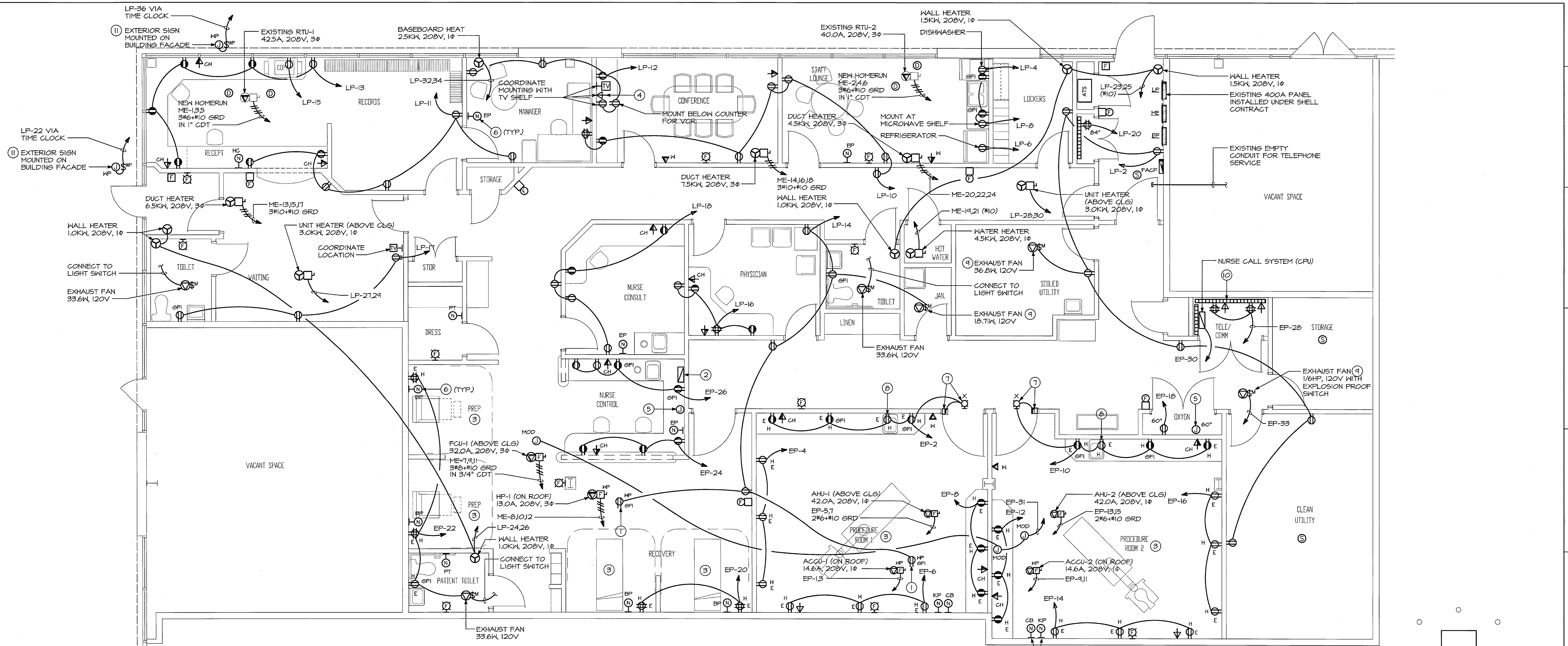
FLOOR PLAN - POWER SCALE: 1/4"=1'-0"
