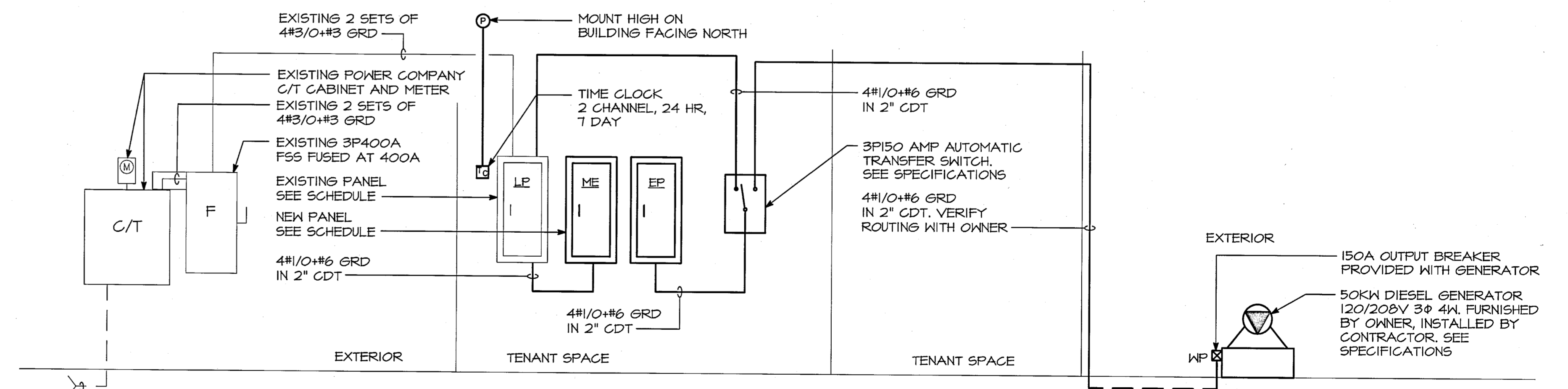
POWER RISER DIAGRAM NO SCALE
