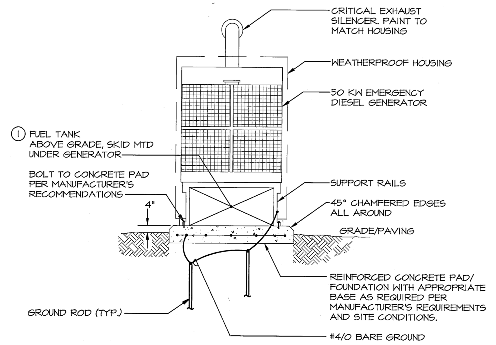
DETAIL - GENERATOR PAD NO SCALE
