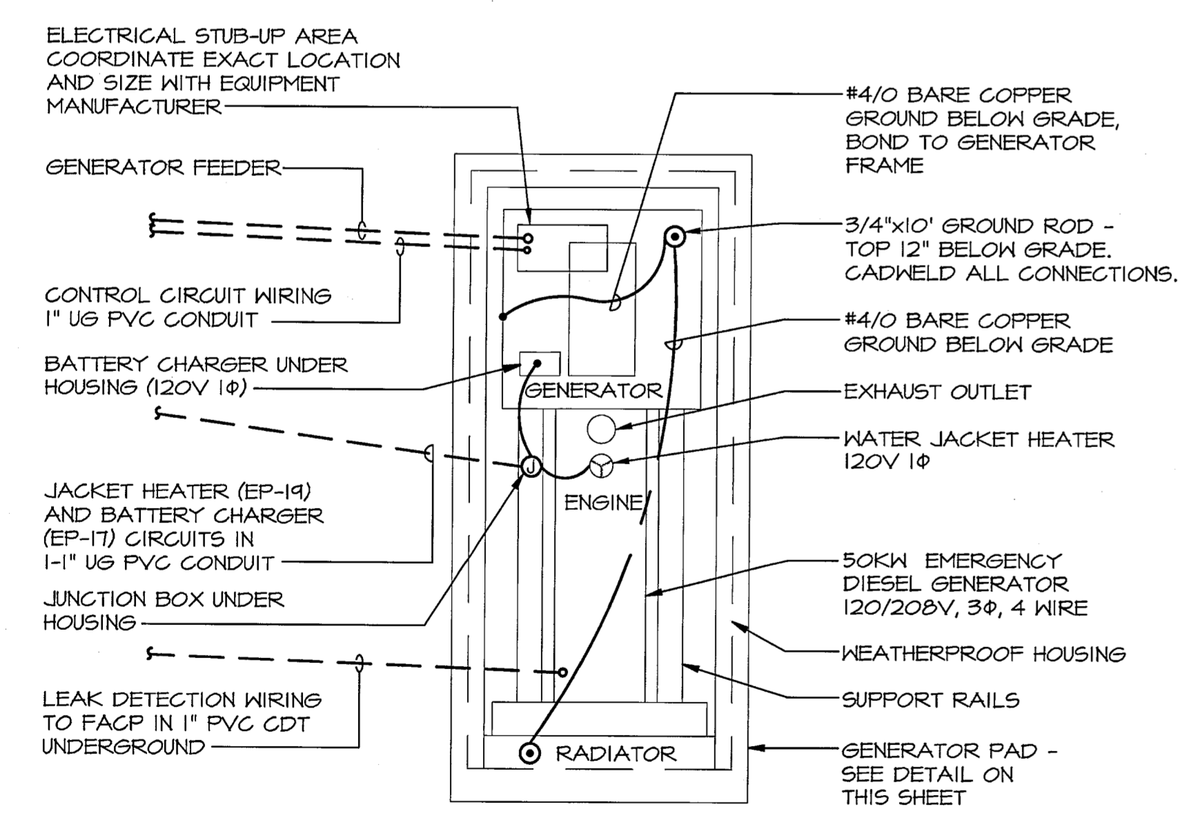
DETAIL - GENERATOR CONNECTIONS NO SCALE
