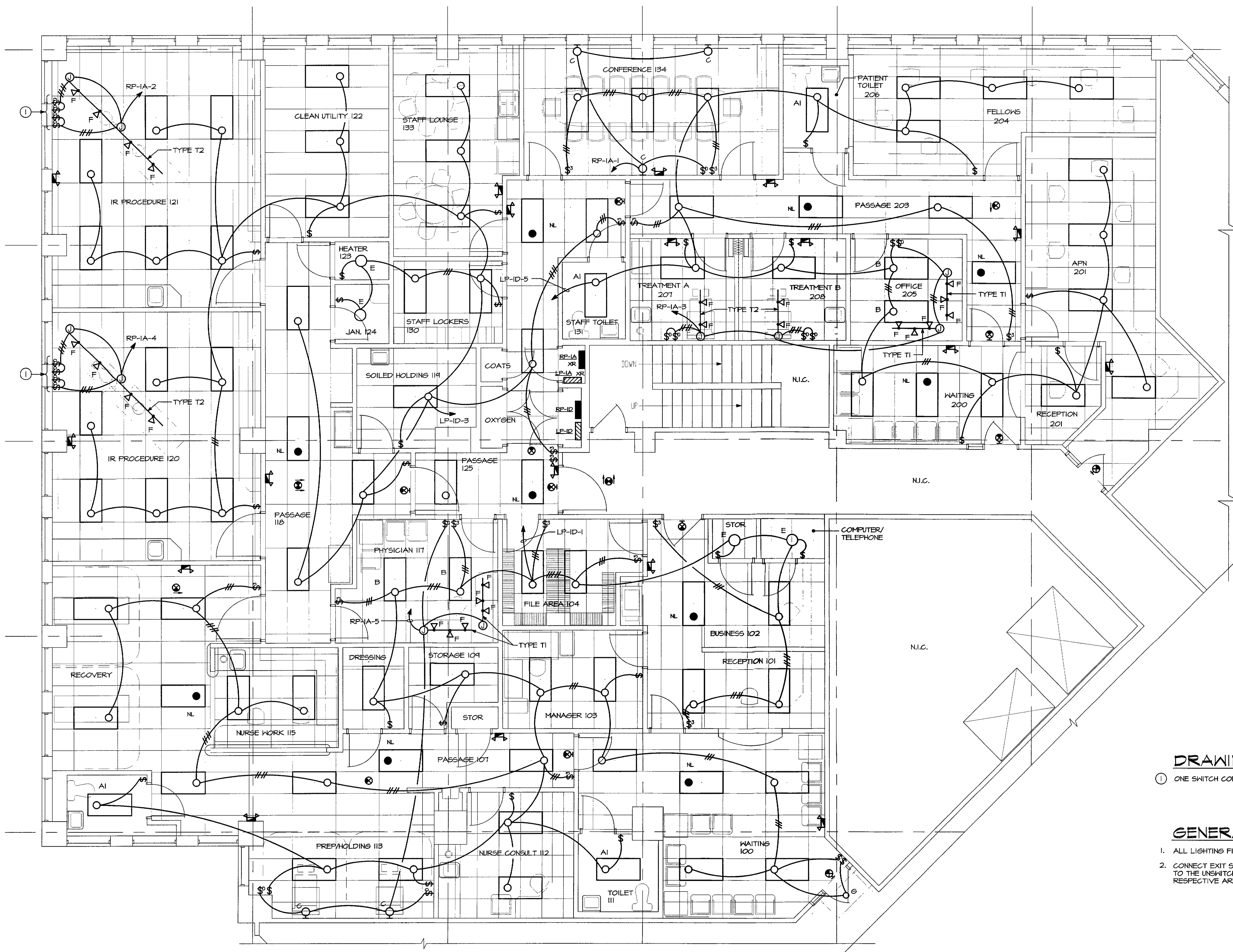
FLOOR PLAN - LIGHTING SCALE: 1/4"=1'-0"
