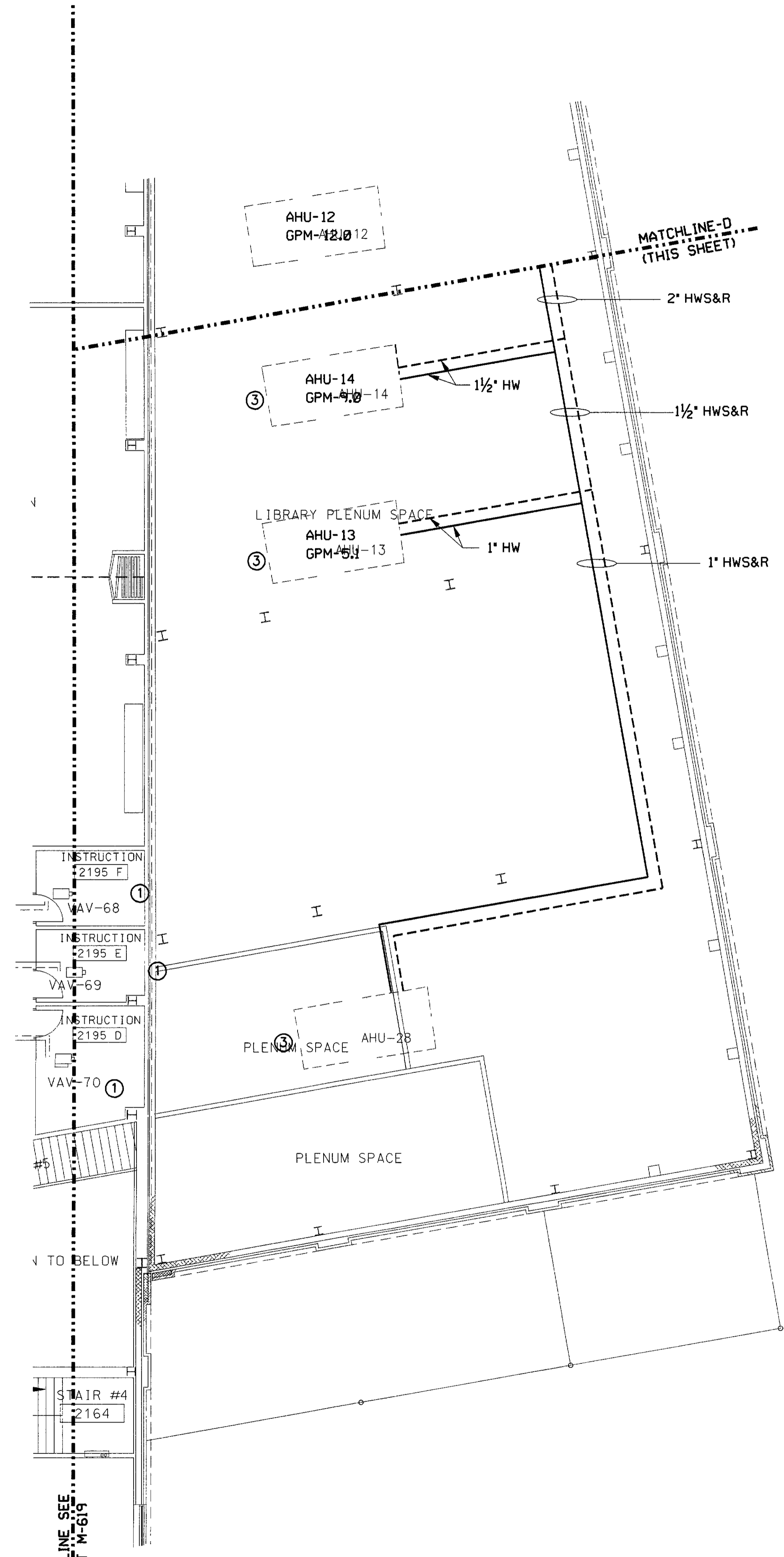
ZONE No. 6 - 2nd FLOOR HVAC PIPING
