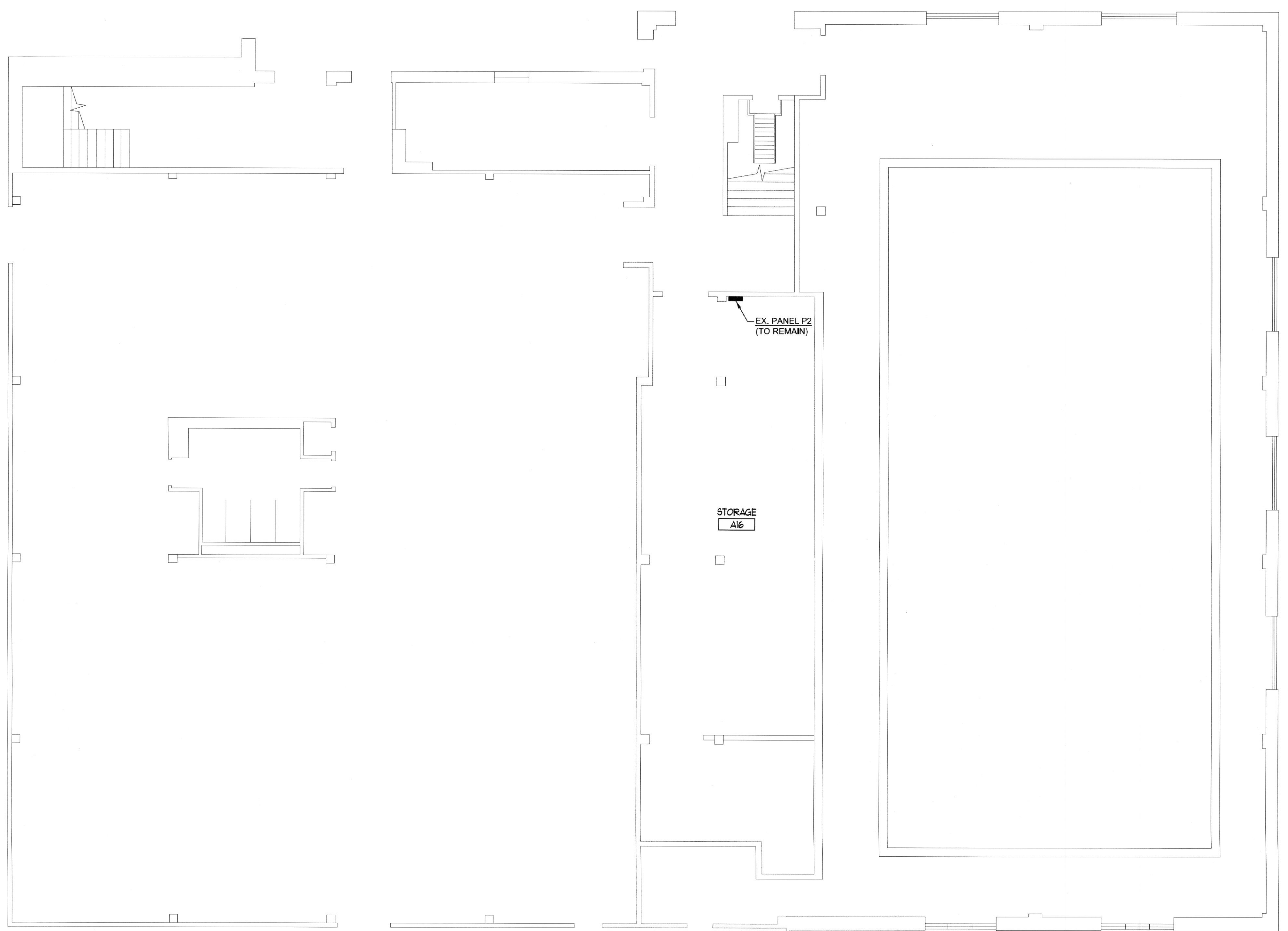
LOWER FLOOR PART PLAN - EXISTING CONDITIONS - ELECTRICAL SCALE: 1/8"=1'-0"
