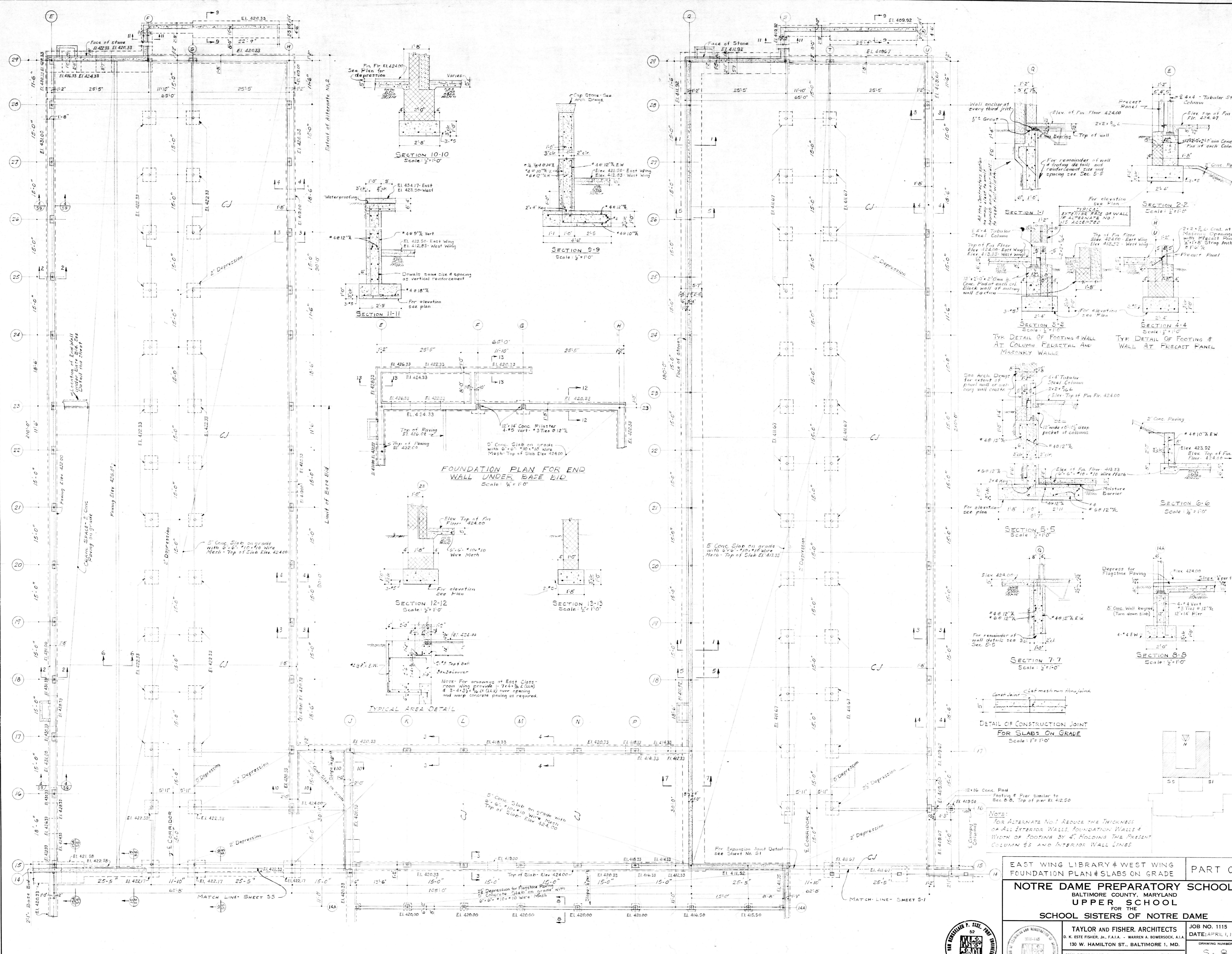
EAST WING, LIBRARY AND WEST WING FOUNDATION PLAN AND SLABS ON GRADE Scale: 1/8" = 1'-0"
