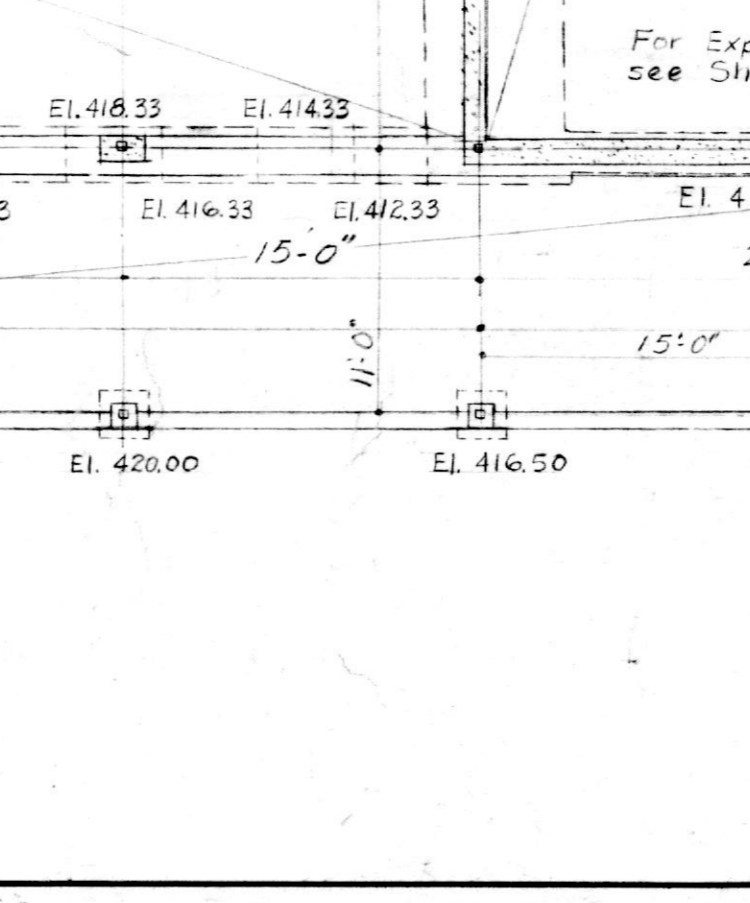
EAST WING, LIBRARY AND WEST WING FOUNDATION PLAN AND SLABS ON GRADE Scale: 1/8" = 1'-0"
