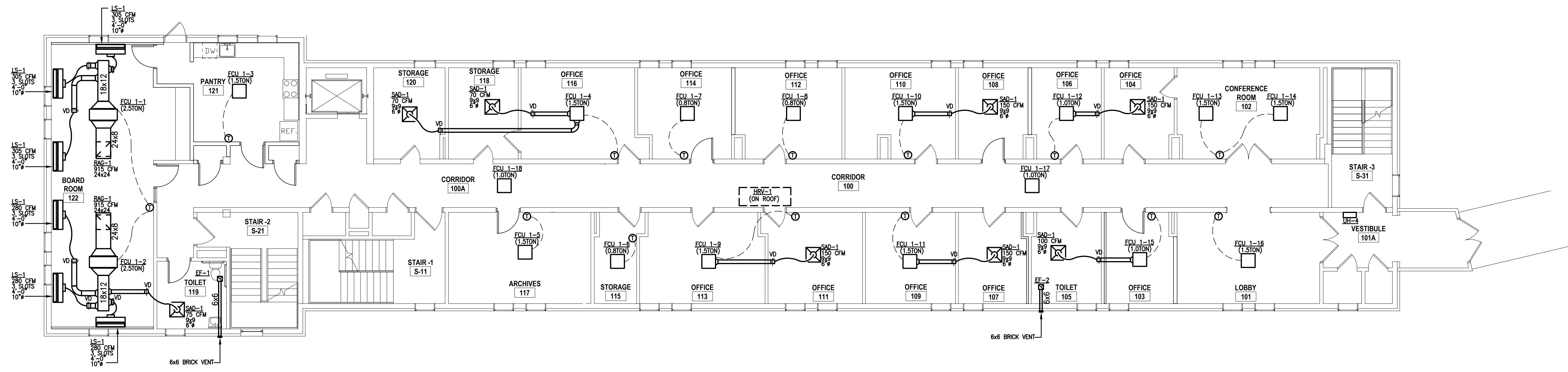
FIRST FLOOR PLAN - HVAC - NEW WORK SCALE: 1/8"=1'-0"
