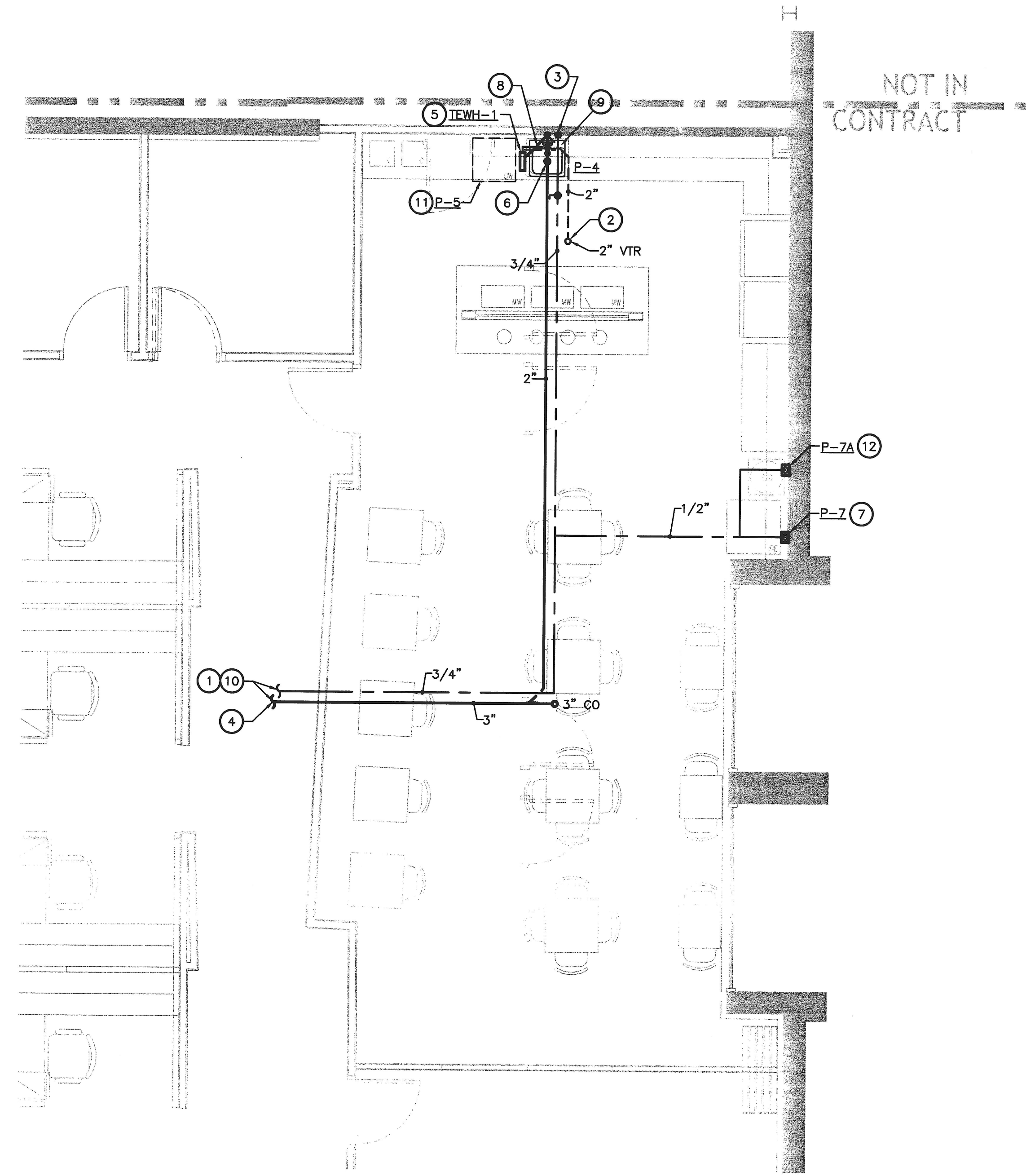
PART PLAN - PLUMBING SCALE: 1/4"=1'-0"
