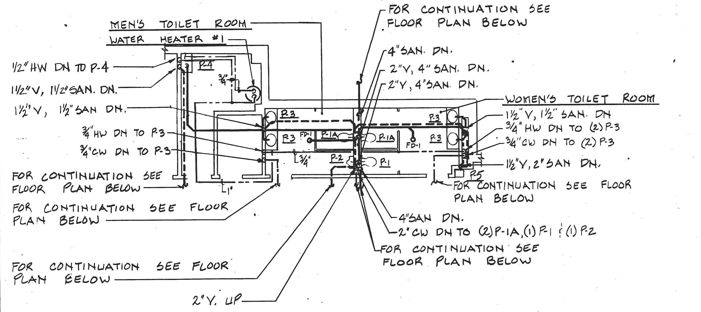
GROUND FLOOR TOILET ROOM - PART PLAN SCALE: 1/8" = 1'-0"
