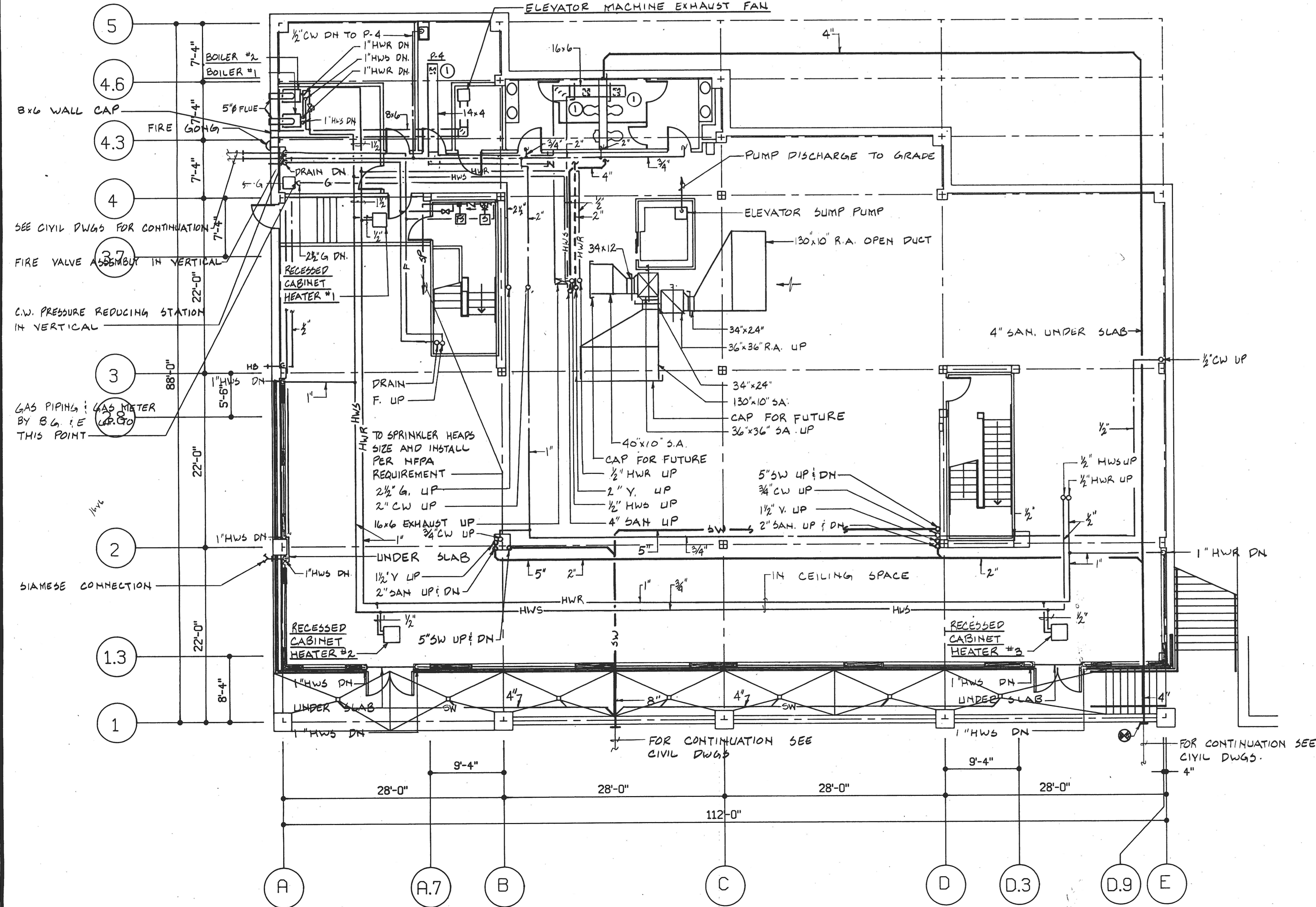
MECHANICAL GROUND FLOOR PLAN SCALE: 1/8" = 1'-0"
