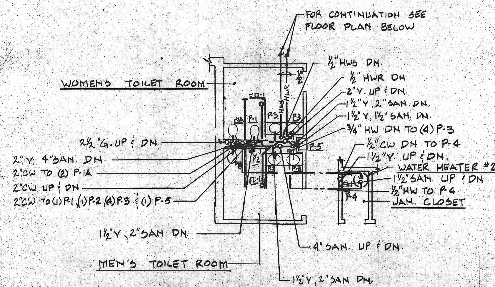
FIRST FLOOR TOILET ROOM - PART PLAN SCALE: 1/8" = 1'-0"
