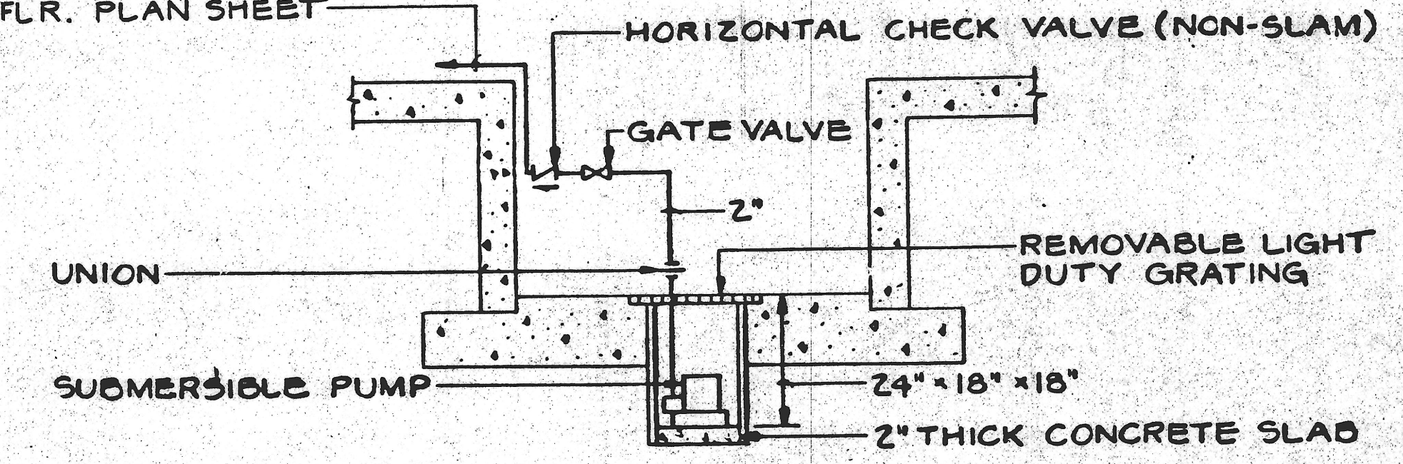
ELEVATOR SUMP PUMP DETAIL SCALE: NONE
