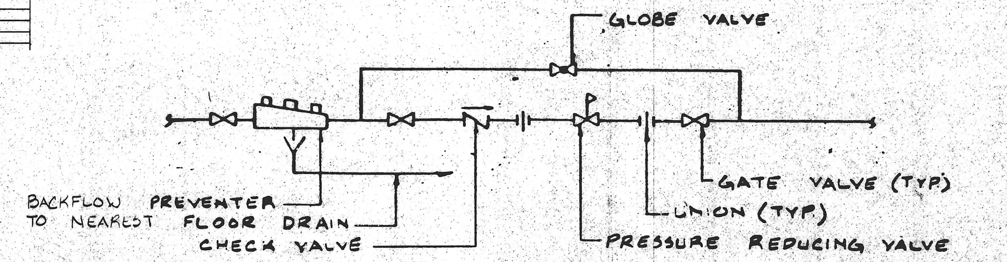
C.W. PRESSURE REDUCING STATION NO SCALE
