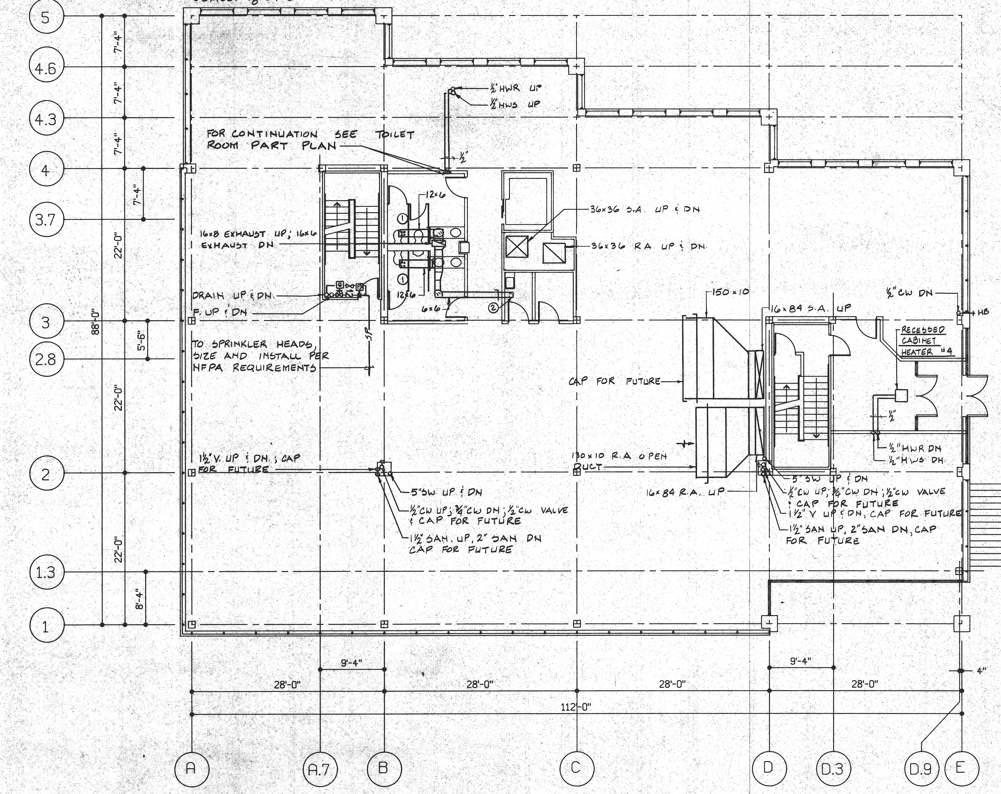
MECHANICAL FIRST FLOOR PLAN SCALE: 1/8" = 1'-0"
