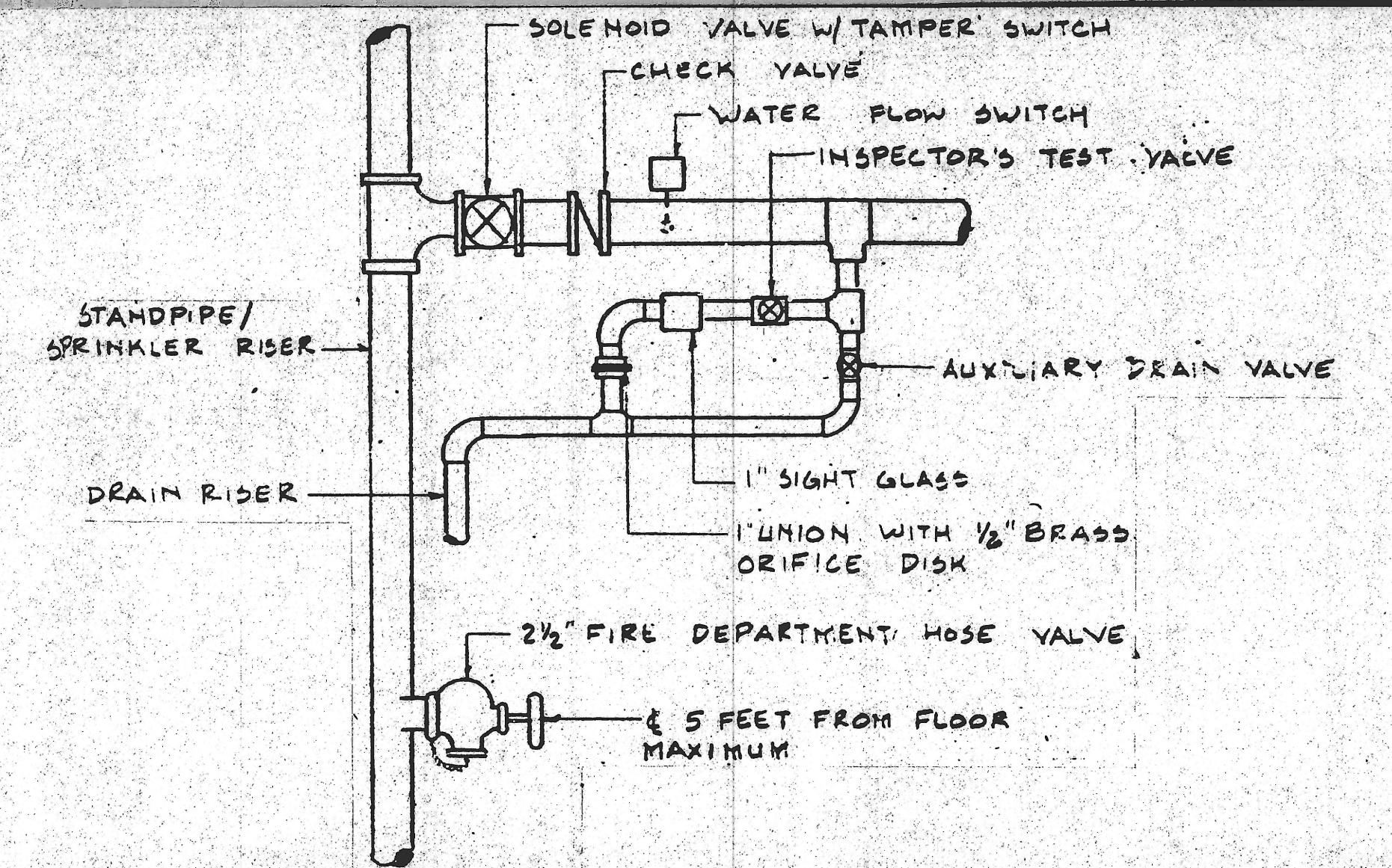
SPRINKLER ZONE VALVE ASSEMBLY DETAIL SCALE: NONE
