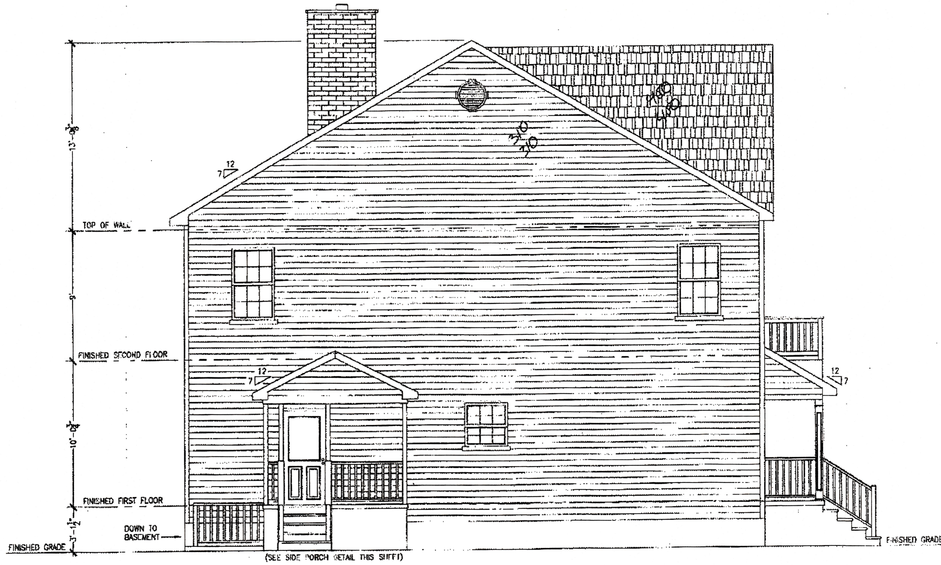
LEFT SIDE FINISHED ELEVATION SCALE: 1/2" = 1'-0"
