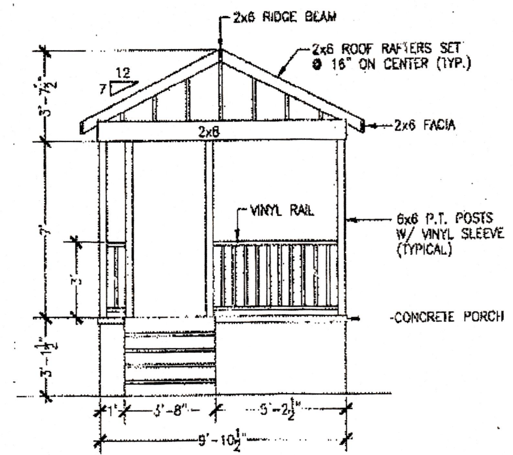
SIDE PORCH DETAIL SCALE: 1/2" = 1'-0"
