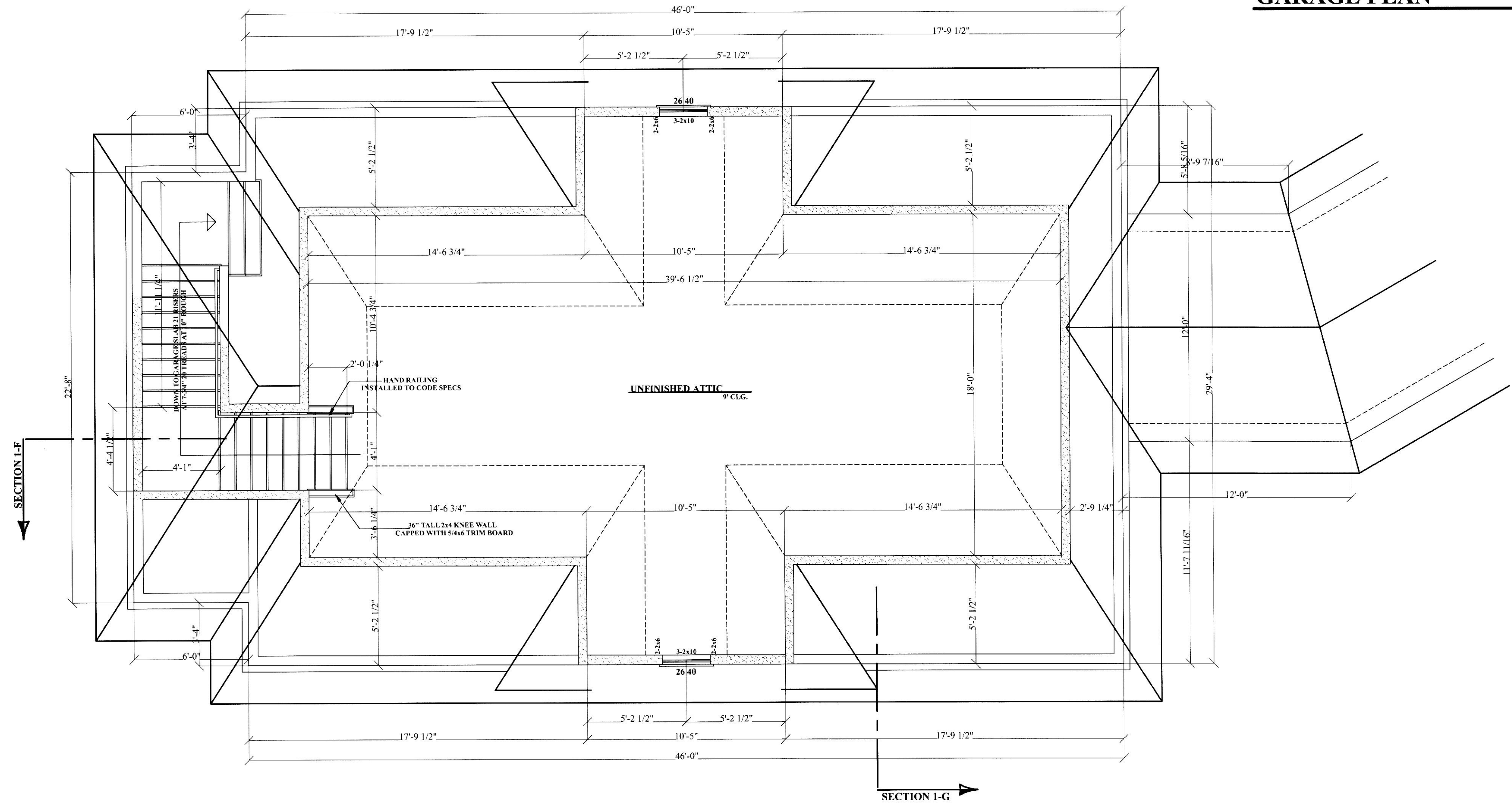
ATTIC FLOOR PLAN
