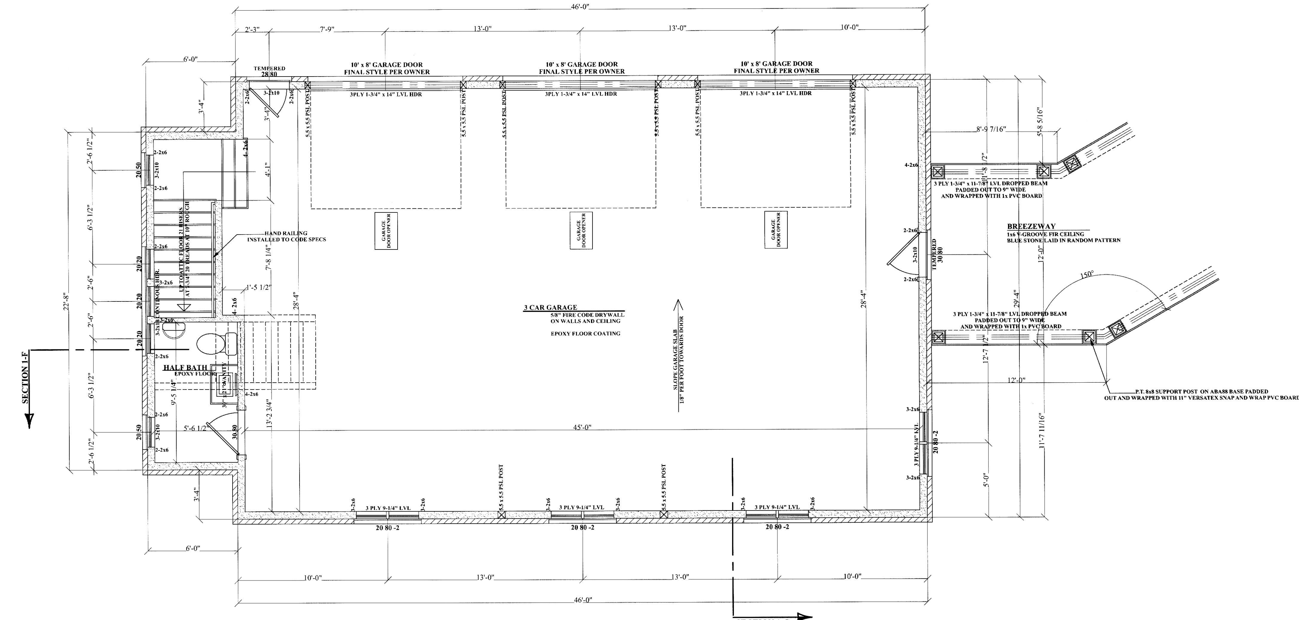
GARAGE PLAN
